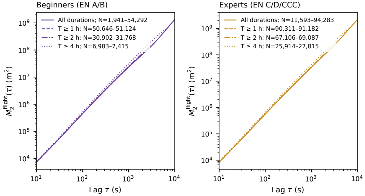
Figure 3.20. The duration comparison repeated for beginners (EN A/B) and experts (EN C/D/CCC), using the same estimator, lag limits and minimum support as Fig. 3.19. Counts refer to distinct flights, and overlapping groups do not constitute independent samples. Tandem, non-certified and unknown equipment is omitted from this contrast.
