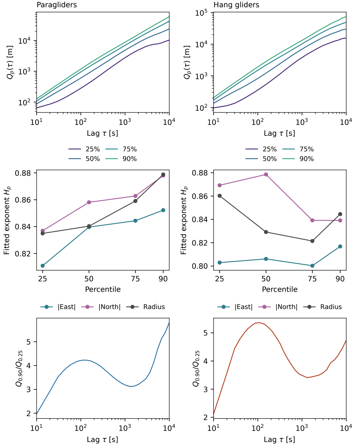
Figure 3.4. Displacement quantiles in the eligible archive over 10 s to 10,000 s, with east and north treated separately from radial displacement. Exponents at individual probability levels and ratios of radial quantiles test whether one scale factor suffices. A common exponent would preserve the quantile ratios; a systematic change indicates shape evolution or a change in the sampled population.
