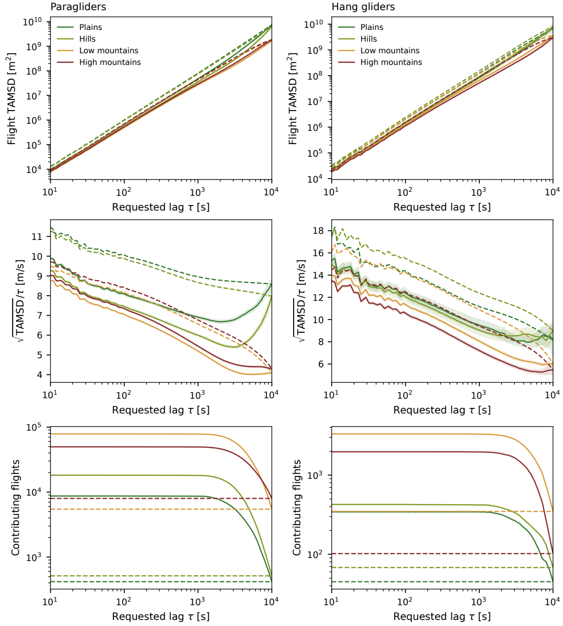
Figure 3.15. The same TA-MSD estimators grouped by cleaned GNSS origin altitude. The names Plains, Hills, Low mountains and High mountains denote the stated altitude bands, not measured terrain classes. All eligible regions enter this grouping. Lines, shading and support conventions match Fig. 3.14.
