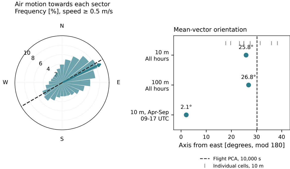
Figure 3.20. ERA5 coastal wind reference and the paraglider covariance axis at 10,000 s. Left: weighted frequency of air motion towards 15-degree sectors at 10 m, excluding speeds below 0.5 \text{ m s}^{-1} and normalising the retained observations. The coloured arrow is the mean wind vector direction, calculated using all hours; the dashed line is the undirected flight axis. Right: mean-vector axes for the annual 10 m reference, an annual 100 m check, and a 10 m April–September, 09–17 UTC check. Grey marks show the nine separate annual cell means, not confidence limits. The same 1,680 coastal flights define the PCA reference in all three comparisons.
