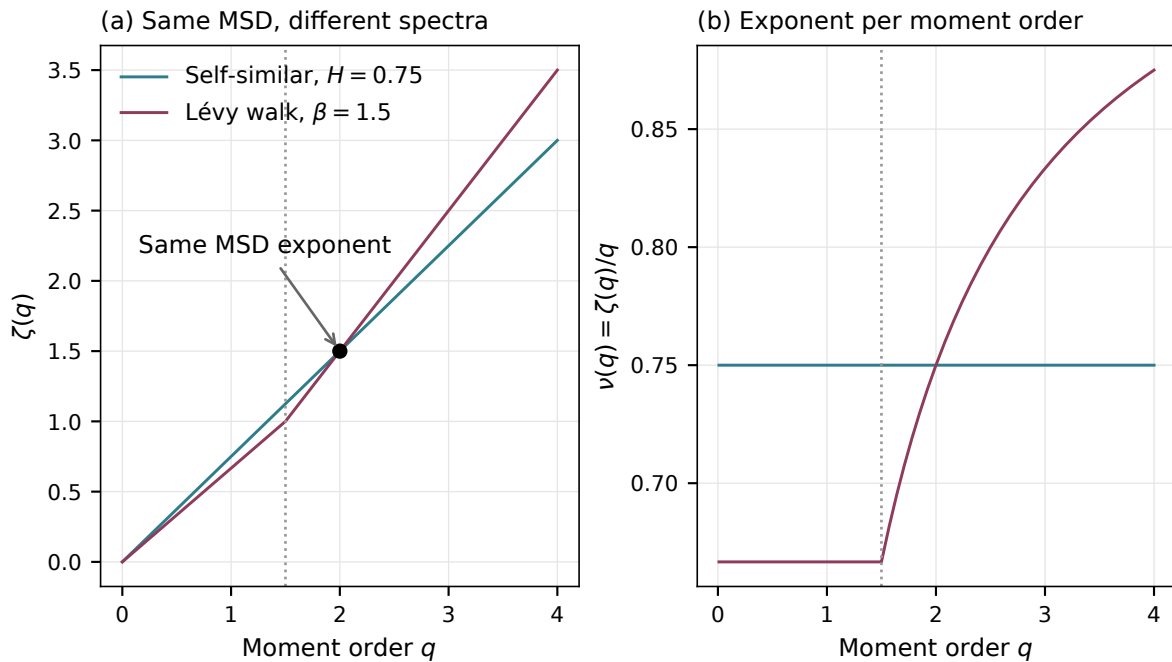
Figure 3.33. Theoretical comparison. A self-similar process with H = 0.75 and a standard Lévy walk with \beta = 1.5 have the same MSD exponent, \zeta(2) = 1.5 , but different moment spectra. The dashed vertical line marks q = \beta . These are asymptotic predictions, not simulated or empirical estimates.
