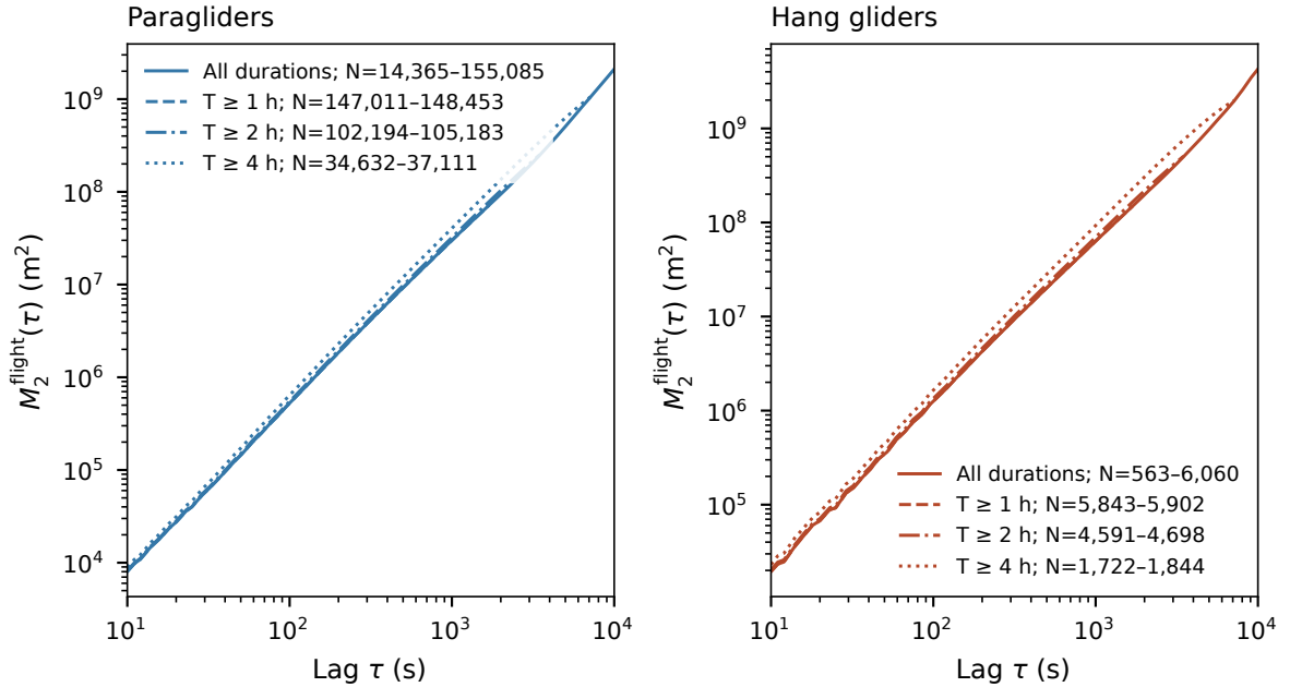
Figure 3.30. Time-averaged squared displacement by retained flight duration. Cohorts are nested; legend counts give the range of contributing flights. Each lag requires at least 30 flights. Threshold curves end at T_0/2 , while the all-duration curve extends to 10,000 s. Shorter flights progressively leave the reference near T_0/2 , bringing the populations closer by selection.
