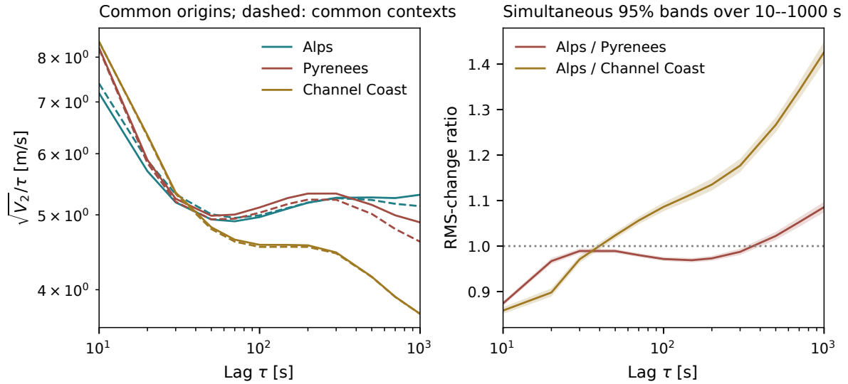
Figure 3.26. Paraglider population controls. Left: common-origin curves, with the common-context standardisation dashed. The dashed curves are descriptive point estimates. Right: regional ratios of the unstandardised common-origin curves; shading is simultaneous over the 18-lag grid's supported subset through 1000 s. These controls do not match meteorology, local terrain exposure or pilot identity.
