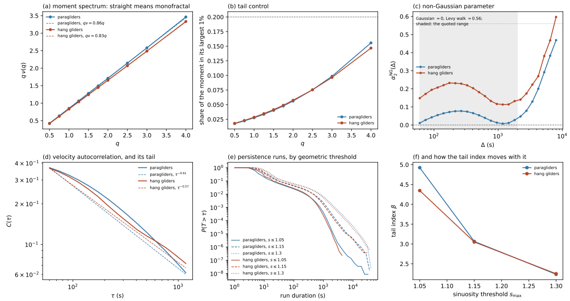
Figure 3.3. What the second moment cannot say. (a) The moment spectrum qv(q) with the straight line qv = \nu q dashed: straight means one exponent governs every moment, and a Lévy walk would bend here with a knee at its tail index. (b) The share of each moment carried by the largest 1% of its increments; above the dashed line a moment is being set by a handful of flights. (c) The non-Gaussian parameter against lag, with the Gaussian value and the Lévy-walk calibration marked and the quoted range shaded; it is flat and clearly above zero inside that range and climbs outside it, where the declared task governs the trajectory. (d) The velocity autocorrelation, log-log with the fitted tail dashed: positive throughout, below 1/e within the first two lags of the grid — whose lower end is the smoothing scale rather than a property of the flying — and decaying too slowly to be integrable. (e) Survival of the persistence-run durations at three geometric thresholds; that they do not lie parallel is the statement that no run length is distinguished. (f) The same thing as one number: the fitted tail index against the threshold that defines a run. Computed by scripts/reporting/generate_shape_figure.py .
