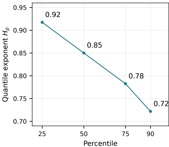
(c) Quantile exponents
