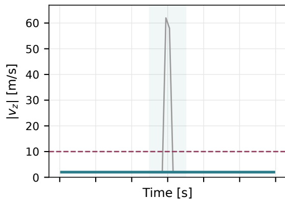
(f) Step and window speeds
