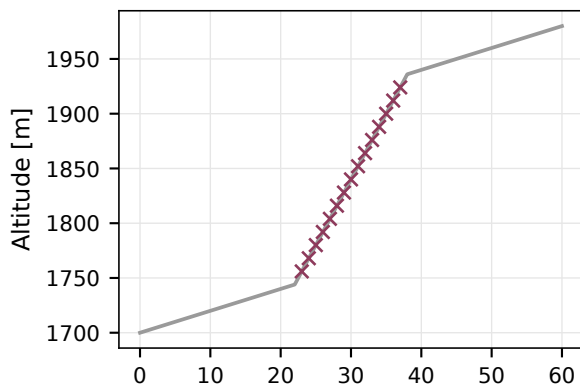
(e) Sustained excess
