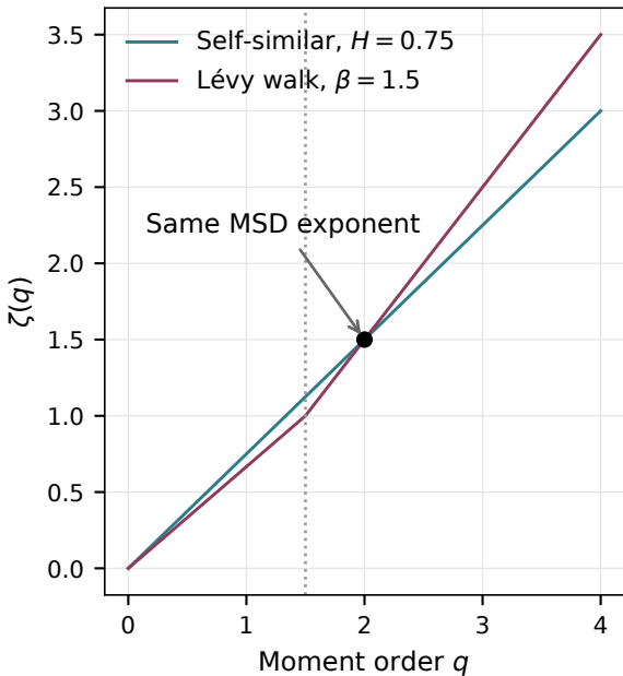
(a) Same MSD, different spectra
