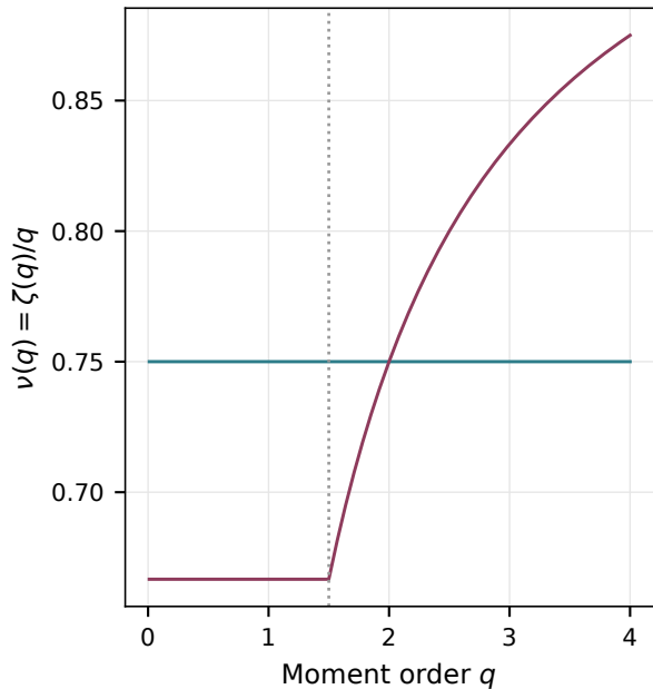
(b) Exponent per moment order
