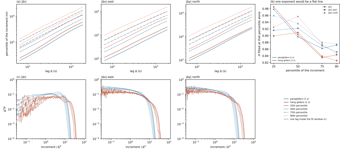
Figure 3.5. The exponent read from the distribution of the increments. All seven panels use each discipline’s fastest native cadence, 1 s, where the histograms hold the most increments. (a) The 25th, 50th, 75th and 90th percentiles against lag, log–log, over the fit window 60 s to 2,000 s, one column for the modulus |\Delta \mathbf{r}| and one for each horizontal component. Four parallel lines would mean one exponent describes every part of that column’s distribution. (b) The slope of each of those four lines, fitted separately, with the modulus and the two components overlaid in one panel. A flat line would mean the same thing as in (a). All three fall from the 25th percentile to the 90th, so the disagreement is not a property of one direction. (c) The histograms behind each column of (a), rescaled by \Delta^H , one curve per lag inside the fit window and every third lag drawn. H = \alpha_2/2 is not a new fit of these histograms: it is the second-order filtered-variation exponent of Table 3.7, reused here rather than re-measured so that a collapsed panel and a quoted exponent never disagree about what H is. For paragliders that is 1.009 (modulus), 0.996 (east), 1.021 (north), and correspondingly 0.972, 0.958, 0.984 for hang gliders.
