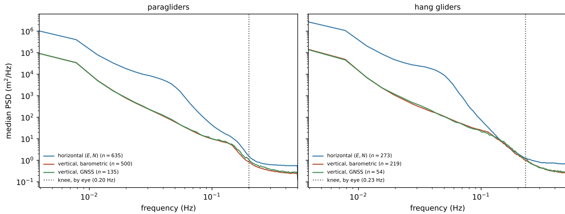
Figure 2.9. The ensemble Welch power spectral density of each channel, by discipline: horizontal ( E, N pooled), barometric-vertical and GNSS-vertical. Median over a seeded sample of up to 900 flights per discipline, restricted to those within 0.25 s of the dominant 1 Hz cadence so every spectrum shares one frequency grid; the usable count per channel is in its legend entry. The dotted line is the knee frequency read by eye off the curves, not fitted: 0.20 Hz for paragliders, 0.23 Hz for hang gliders. Within a panel the three channels flatten into the same floor at visibly the same frequency; paragliders and hang gliders fly at very different speeds, yet the two panels' knees still land within a few hundredths of a hertz of each other, the cross-check the main text draws on.
