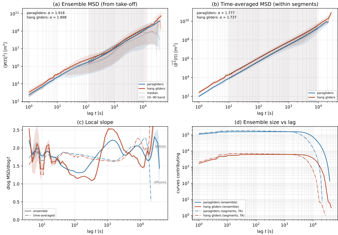
Figure 3.1. Mean-squared displacement of the retained ensemble, by two averages, each with its own fitted power law and fitted range, one dashed line and one shaded band per discipline. (a) Ensemble MSD against elapsed flight time, log–log, 10 % to 90 % band across flights. (b) Time-averaged MSD, cut at half a segment’s length. (c) Local logarithmic slope of both: a windowed Theil–Sen estimator, the median of the pairwise log–log slopes between every pair of grid points within \pm 0.15 decades of a lag (five to six points on this grid), banded by the interquartile range of those pairwise slopes over 1.349\sqrt{N} (implementation details: Sec. I3); ballistic and diffusive values marked. (d) Flights contributing at each lag, which sets the upper end of each fit range.
