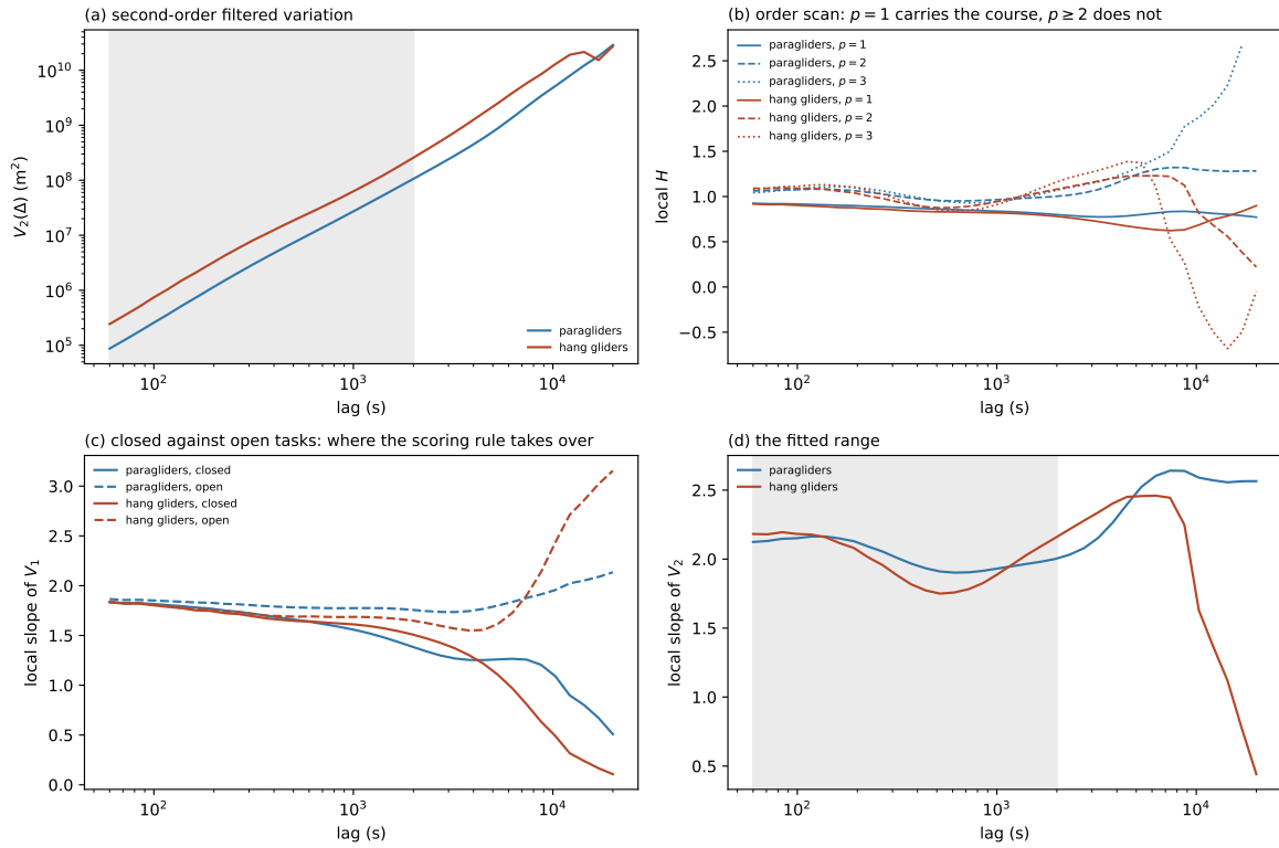
Figure 3.3. The filtered variation, on which the exponent is read. (a) V_2(\Delta) against lag, log–log, fitted range shaded. (b) Local H = \frac{1}{2} d \log V_p / d \log \Delta at the three filter orders: p = 1 runs below p = 2, 3 , the flown course read as a lower exponent. (c) Local slope at p = 1 split by declared task; closed and open courses part company past 3,000 s. (d) Local slope of V_2 , the quantity the fit averages.
