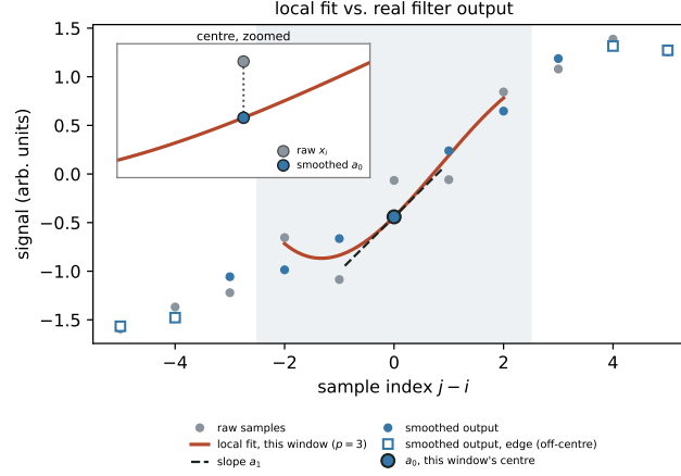
Figure 2.8. The Savitzky–Golay filter as a local fit and as a fixed convolution, on a synthetic series, \sin(0.28j) + \varepsilon_j with i.i.d. Gaussian noise \varepsilon_j \sim \mathcal{N}(0, 0.35^2) (dots). The highlighted window's own local cubic fit (thick line), and the values it reads off at its centre, a_0 (ringed dot) and the slope a_1 (dashed); the inset zooms on the centre, where the fit trades the one raw sample x_i (grey) for the smoothed a_0 (blue). Alongside it, the actual filtered output run on the whole span exactly as the filter runs it on a flight segment. The m points nearest each edge (hollow squares) have no full window on one side, so they are fitted on the nearest full window inside the span and evaluated off-centre.
