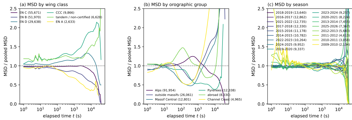
Figure 3.4. Whether the retained ensemble may be pooled: the ensemble MSD computed within each stratum and divided by the pooled curve, for paragliders, (a) by wing class, (b) by orographic group and (c) by season; strata below 2,000 flights are not drawn. Class and terrain separate the curves, season does not.
