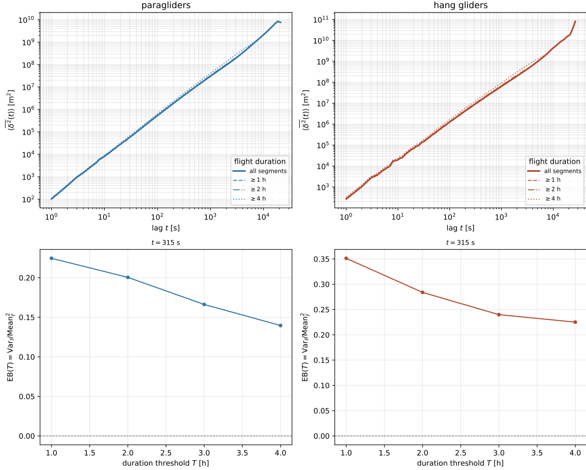
Figure 3.2. Two readings of the same question. (a) The time-averaged MSD of Figure 3.1b ( all segments ) beside its own fixed-duration cohorts, each cut at half its own threshold: coinciding curves would say the time average does not depend on the duration of the record it is read from, and on this archive they separate by tens of per cent, too little to see against eight decades of growth. (b) EB(T) , App. 3.A’s ergodicity-breaking parameter, measured directly from the scatter of each flight’s own time average (Sec. 3.2’s V_1 ) rather than proxied by panel (a)’s duration split, at one lag held fixed (315 s) and swept over the duration threshold T – the dependence App. 3.A defines the parameter to test, not its dependence on the lag: zero (dashed) is the ergodic limit, and a curve that falls with T without reaching it is a weakening rather than a vanishing of the aging signature read off the archive’s own flights.
