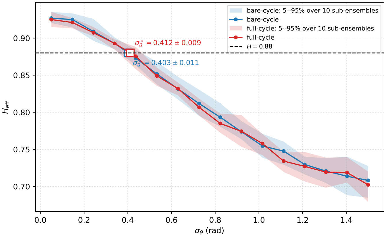
H_{\text{eff}}(\sigma_\theta) — paragliders (fit window [10, 7000] s)
