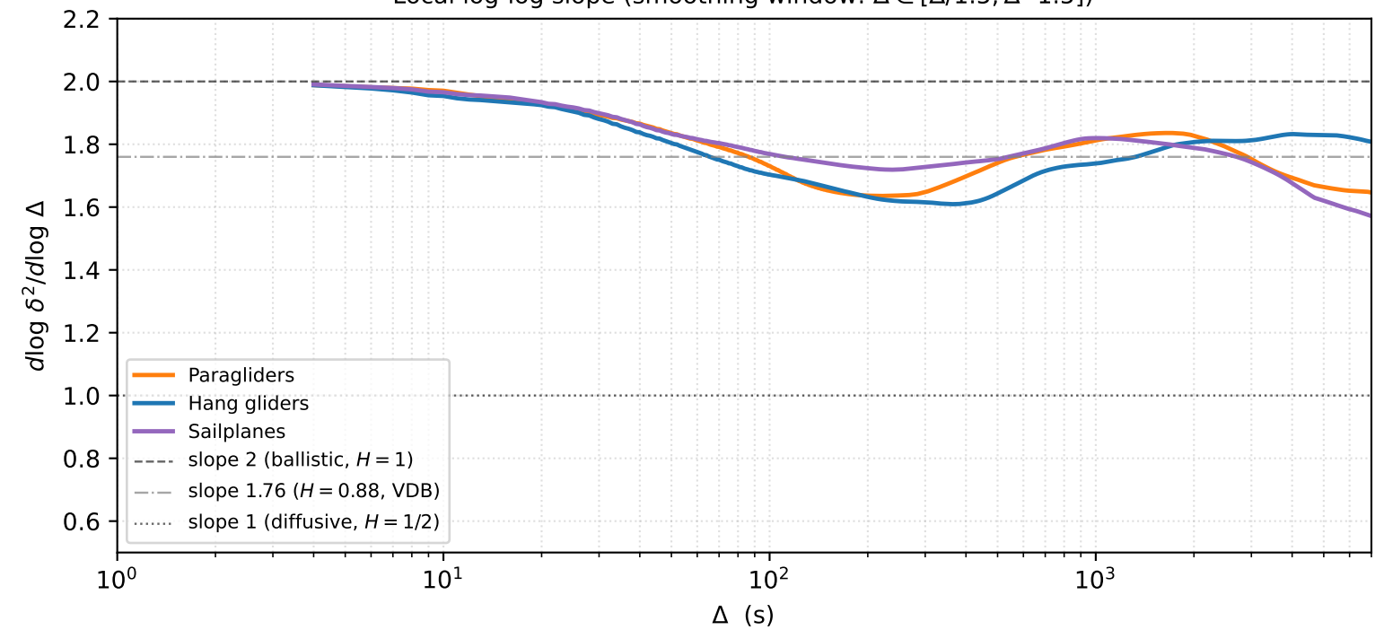
Local log-log slope (smoothing window: \Delta \in [\Delta/1.5, \Delta \cdot 1.5] )
