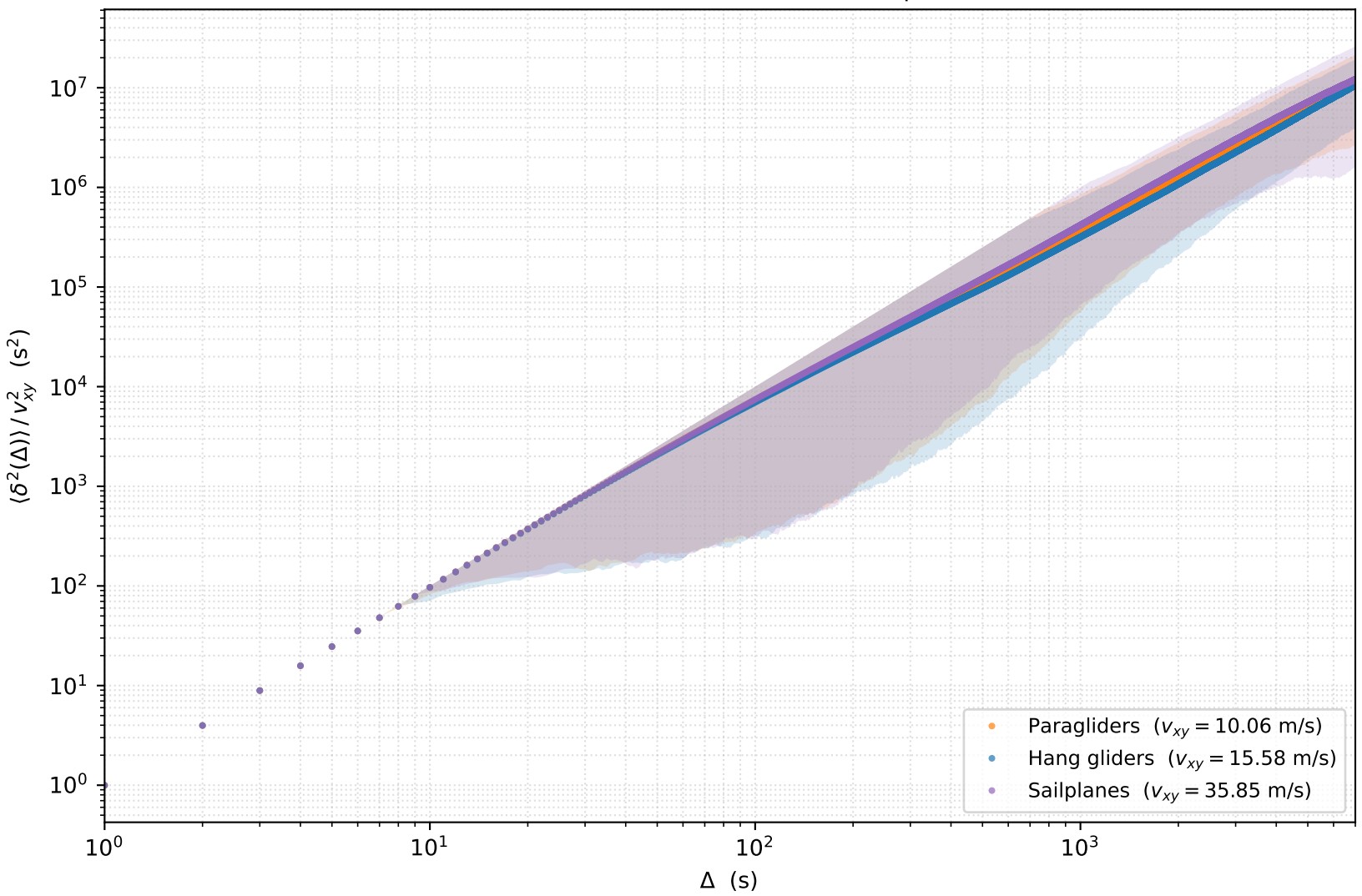
Rescaled MSD — universal collapse
