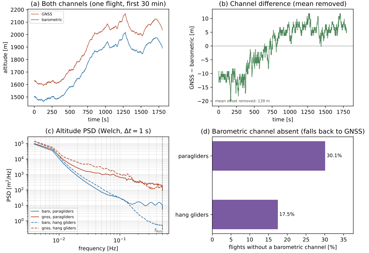
Figure 4.1: Barometric vs GNSS altitude noise. For one representative flight (the one with the most fixes in the subsample), over the same 30 min window: (a) the two raw channels overlaid on one shared y -axis. The two curves start about 130 m apart and separate further as the flight climbs – that growing gap is the point of this panel, so nothing here renormalises it away; it is not, however, where the claim that GNSS is the noisier channel rests – at this timescale a climb of hundreds of metres dwarfs a jitter of a few metres on the plotted scale, so a single flight’s raw trace is the wrong place to look for it; that evidence is panel (c). (b) Their difference GNSS–barometric (mean removed, not detrended): the same growing gap as in panel (a), quantified. That drift, of order several tens of metres over the window, is a real, physically meaningful feature – plausibly the barometric channel’s progressive departure from the ICAO standard atmosphere as altitude changes – not noise to be filtered out, so only the constant part of the offset is subtracted; its value for this flight (139 m) is annotated on the panel, matching the vertical gap seen directly in panel (a). Over the ensemble: (c) mean Welch power spectra of the two channels, per discipline (Appendix B; 212/400 paraglider and 114/400 hang-glider sampled flights actually contribute, after the common-cadence selection described there) – here, and only here, does the two-to-three-orders-of-magnitude gap between the channels at high frequency make the noise-floor claim; the dotted line is the Nyquist frequency f_{\text{Nyq}} = 1/(2\Delta t) , the highest frequency the sampling can resolve. It is a single line because the pooled flights are all resampled to the same modal \Delta t before averaging, so they share one \Delta t – hence one f_{\text{Nyq}} . (d) Fraction of flights whose barometric channel is absent, per discipline; see the main text for how these were measured and their precision.
