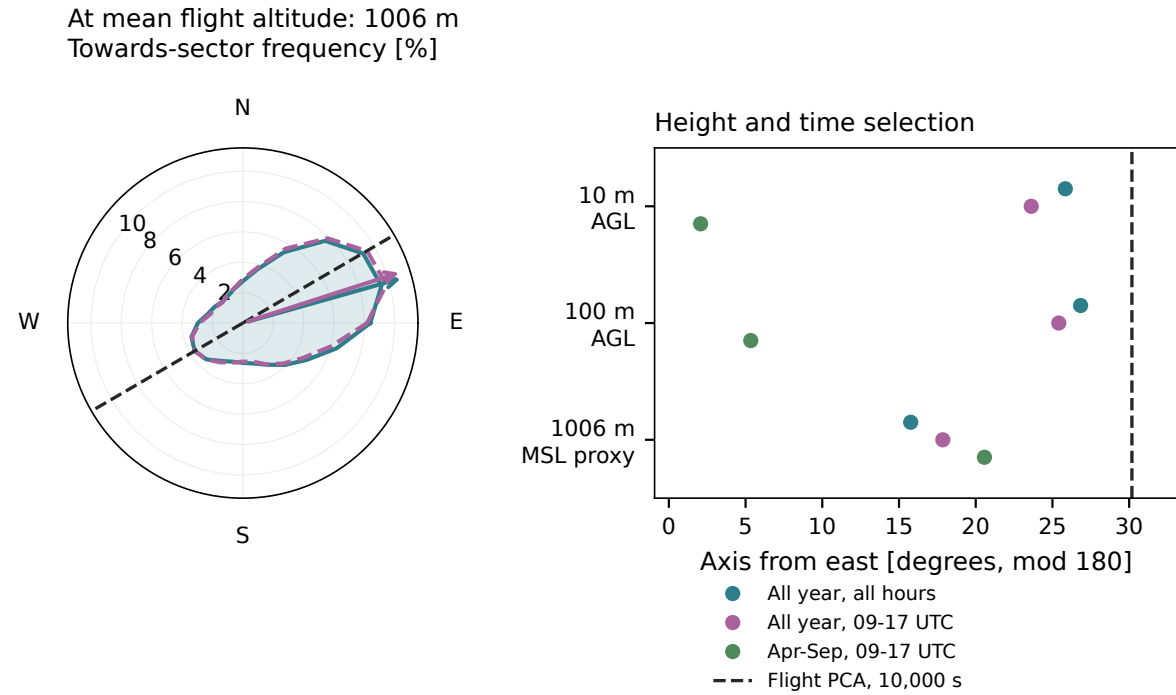
Figure 3.20. ERA5 wind at mean coastal flight altitude and the paraglider PCA at 10,000s. Left: frequencies of air motion towards 15-degree sectors at 1,006 m, for all-year all hours and all-year 09–17 UTC. Speeds below 0.5 \text{ m s}^{-1} are excluded only from the frequency curves; arrows show the vector means using all selected hours. Right: wind axes at flight altitude, approximately above mean sea level, and at 10 and 100 m above ground (AGL). The warm daytime selection is shown as a separate check. The dashed black line is the same flight covariance axis in every comparison.
