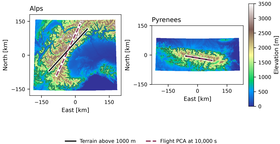
Figure 3.19. Independent terrain orientation compared with the paraglider displacement covariance at 10,000 s. Elevation and the 1,000 m contour come from ETOPO 2022 [26]. The solid dark line is the highland-footprint axis; the dashed coloured line is the flight PCA axis, translated to the same centre for comparison. Line lengths carry no displacement or ridge-length information. Map coordinates are kilometres east and north of each box centre.
