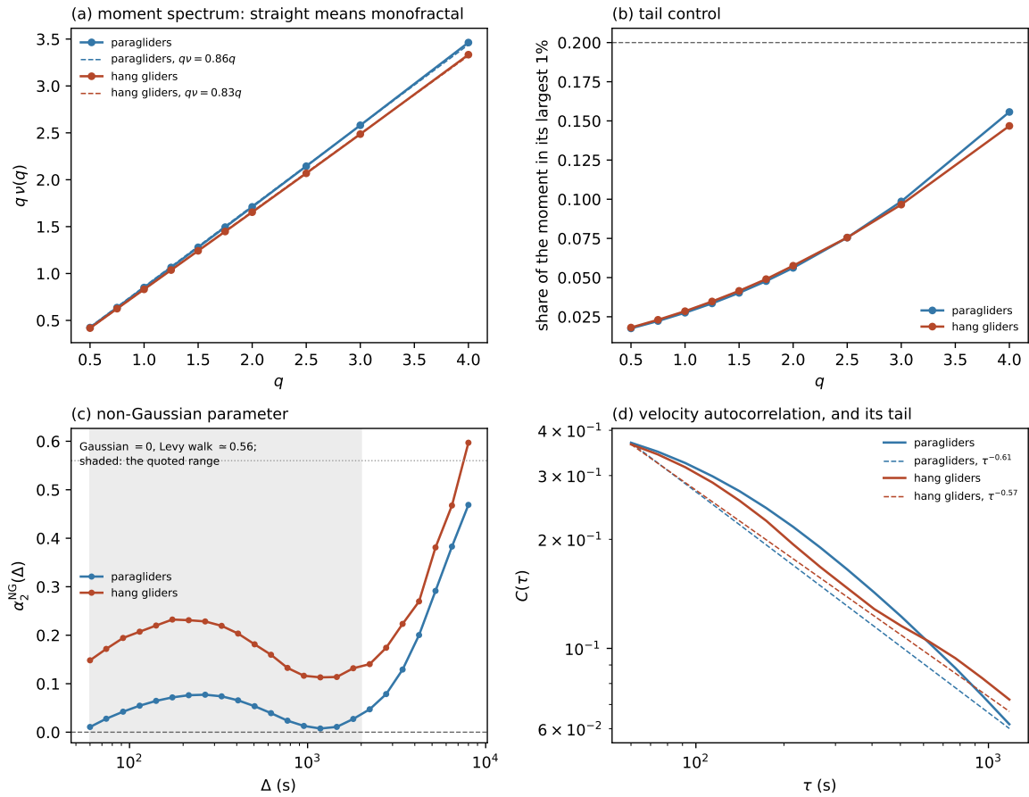
Figure 3.4. What the second moment cannot say. (a) Moment spectrum q\nu(q) , straight line dashed: straight means one exponent for every moment. (b) Share of each moment carried by the largest 1 % of increments. (c) Non-Gaussian parameter against lag, Gaussian and Lévy-walk values marked. (d) Velocity autocorrelation, log-log, fitted tail dashed.
