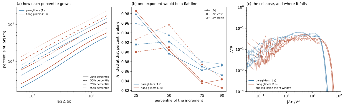
Figure 3.3. The exponent read from the distribution of the increments, not from a moment of it. All three panels use each discipline’s fastest native cadence, 1 s, where the histograms hold the most increments. Panels (a) and (c) use the modulus |\Delta \mathbf{r}| ; panel (b) sets it beside the two components. (a) The 25th, 50th, 75th and 90th percentiles of |\Delta \mathbf{r}| against lag, log–log, over the fit window 60 s to 2,000 s. Four parallel lines would mean one exponent describes every part of the distribution. (b) The slope of each of those four lines, fitted separately. A flat line would mean the same thing. The three marker styles are the modulus and the two components; all of them fall from the 25th percentile to the 90th, so the disagreement is not a property of one direction. (c) The histograms behind (a), rescaled by \Delta^H , one curve per lag inside the fit window and every third lag drawn. H is that row’s own value, 0.884 for paragliders and 0.873 for hang gliders. If the scaling form held exactly the curves would lie on top of one another; they do through the bulk and separate at the flanks.
