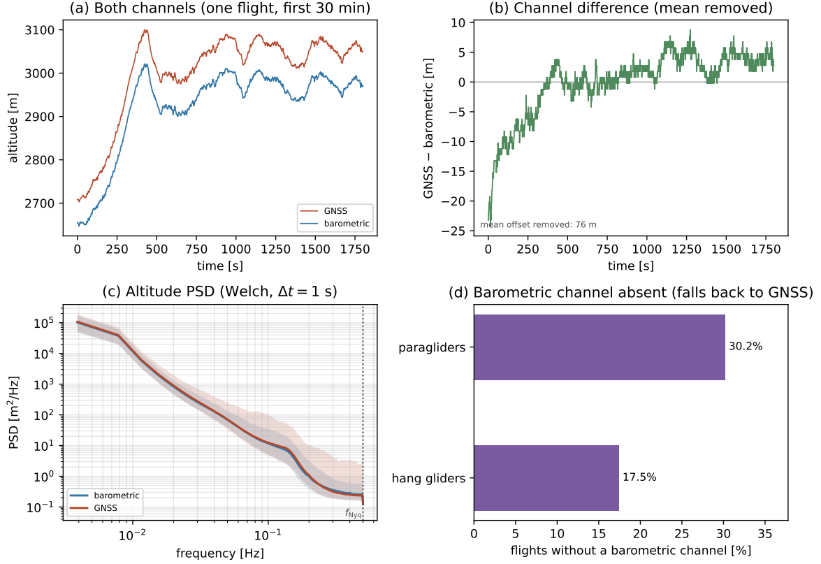
Figure 2.1. Barometric vs GNSS altitude noise. (a) One representative flight over a 30 min window, the two raw channels on a shared axis. The vertical gap between the curves is the offset between their reference surfaces (pressure vs. ellipsoidal). (b) Their difference, mean removed: the offset is not constant but drifts by tens of metres already within this 30 min window. (c) Per-frequency median Welch spectrum of each channel (Appendix 2.A), pooled over the two disciplines, with the 10 to 90 percentile band across flights; the medians nearly coincide, while the GNSS band fans out towards the Nyquist frequency f_{\text{Nyq}} = 1/(2\Delta t) (dotted). The median is used because the per-flight spectra are heavy-tailed (Sec. 2.7.1). (d) Fraction of flights whose barometric channel is absent, per discipline. (implementation details: Sec. 2.7.1)
