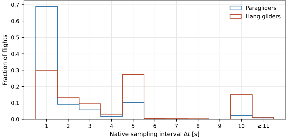
Figure 2.15. Native sampling interval per flight, measured as the median inter-fix time in the raw archive. Bars give the fraction of flights in one-second bins; the last bin also includes intervals beyond 11 s. Paragliders concentrate at 1 s, while hang gliders are spread across several cadences. Resampling preserves each flight’s native interval.
