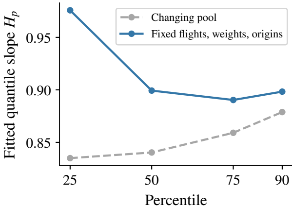
Paragliders ( N_* = 14360 )
