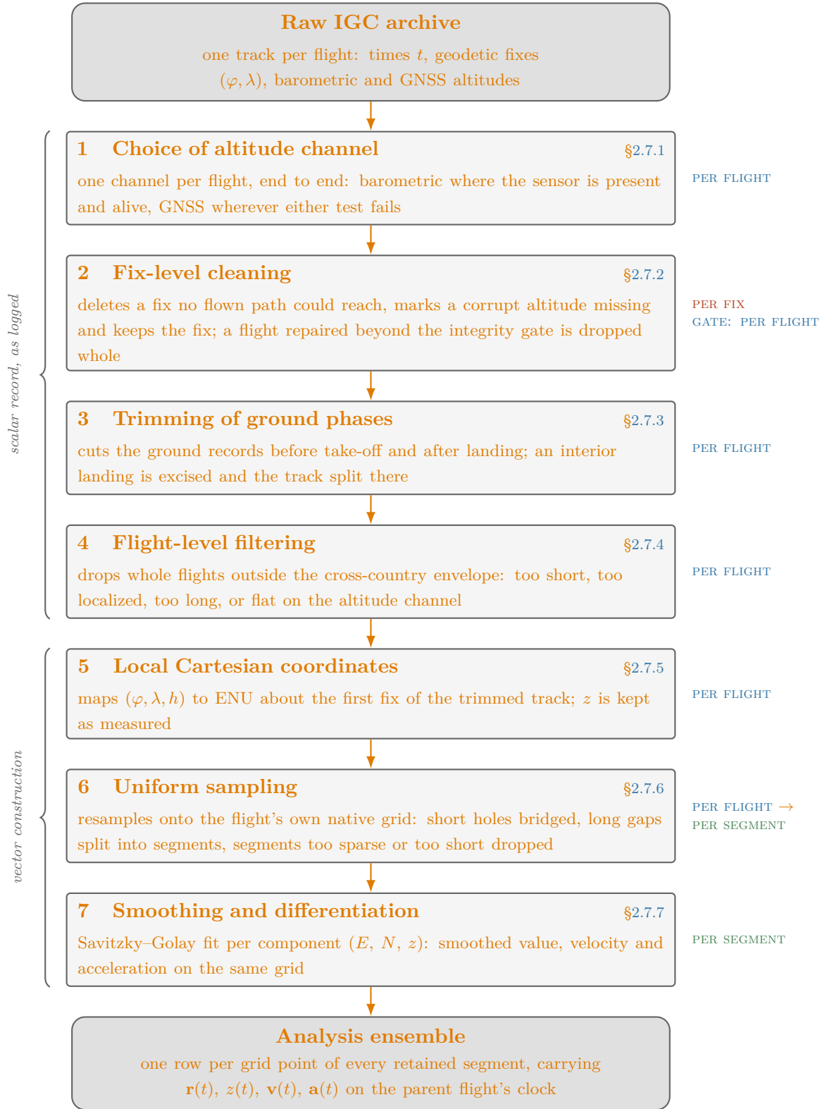
Figure 2.12. The processing chain, from the raw archive to the analysis ensemble. Each stage carries its effect and the section that argues the choice; the badge to the right is the level it acts at (per fix, per flight, per segment). Every check on the scalar record (stages 1–4) precedes the construction of vector quantities (stages 5–7), so no coordinate conversion is computed for a record about to be repaired or dropped. The thresholds each stage applies are listed, with their symbols, in Table 2.7.
