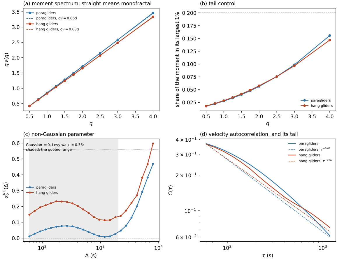
Figure 3.4. What the second moment cannot say. (a) Moment spectrum q\nu(q) , straight line dashed: straight means one exponent for every moment. (b) Share of each moment carried by the largest 1% of increments. (c) Non-Gaussian parameter against lag, Gaussian and Lévy-walk values marked. (d) Velocity autocorrelation, log-log, fitted tail dashed.
