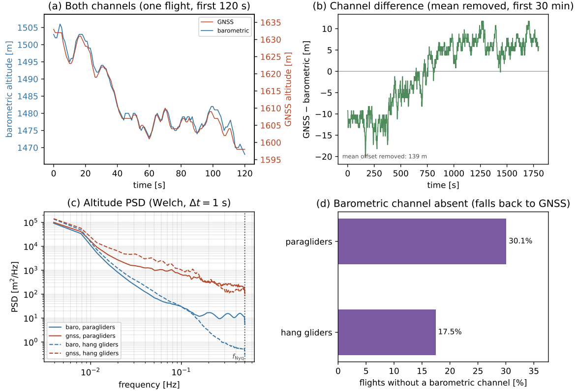
Figure 4.1: Barometric vs GNSS altitude noise. For one representative flight (the one with the most fixes in the subsample): (a) the two raw channels over a short, 120s window – short on purpose, so the jitter is visible at all; over a longer window the altitude excursion itself spans hundreds of metres and swamps a jitter of a few metres on the plotted scale. The two channels are each on their own y-axis (barometric left, GNSS right), with the same numeric span but a different baseline: a shared axis would need to span from one channel’s minimum to the other’s maximum – the real vertical motion plus their mutual offset (of order 100 m, see below) – wasting on blank space the room needed to actually compare the two channels’ roughness. With matched spans, the GNSS trace is visibly more jagged than the barometric one. (b) Their difference GNSS–barometric (mean removed, not detrended) over a much longer, 30 min window: long enough for the slow drift of the offset between the channels to show up alongside the residual jitter. That drift, of order several tens of metres over the window, is a real, physically meaningful feature – plausibly the barometric channel’s progressive departure from the ICAO standard atmosphere as altitude changes – not noise to be filtered out, so only the constant part of the offset is subtracted; its value for this flight is annotated on the panel, to be read alongside the vertical gap between the two curves in panel a. Over the ensemble: (c) mean Welch power spectra of the two channels, per discipline (Appendix B); the dotted line is the Nyquist frequency f_{\text{Nyq}} = 1/(2\Delta t) , the highest frequency the sampling can resolve. It is a single line because the pooled flights are all resampled to the same modal \Delta t before averaging, so they share one \Delta t – hence one f_{\text{Nyq}} . (d) Fraction of flights whose barometric channel is absent, per discipline; see the main text for how these were measured and their precision.
