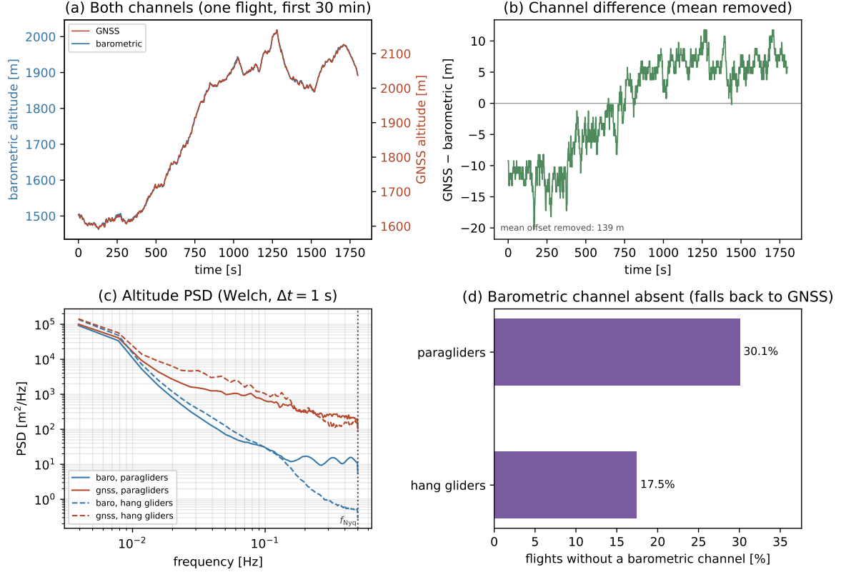
Figure 3.1: Barometric vs GNSS altitude noise. For one representative flight, over the same 30 min window: (a) the two raw channels, each on its own , independently auto-scaled y -axis (barometric left, GNSS right): the two curves then track almost on top of each other, since each is stretched to fill the panel with its own climb – the point of this panel is that shared shape, not their offset (that’s panel (b)’s job). Nor is this panel where the claim that GNSS is the noisier channel rests – a climb of hundreds of metres dwarfs a jitter of a few metres at this timescale, so a single flight’s raw trace is the wrong place to look for it; that evidence is panel (c). (b) Their difference GNSS–barometric (mean removed, not detrended): the offset and its drift, of order several tens of metres over the window, put on a single shared scale. That drift is a real, physically meaningful feature – plausibly the barometric channel’s progressive departure from the ICAO standard atmosphere as altitude changes – not noise to be filtered out, so only the constant part of the offset is subtracted; its value for this flight is annotated on the panel. Over the ensemble: (c) mean Welch power spectra of the two channels, per discipline (Appendix B) – here, and only here, does the two-to-three-orders-of-magnitude gap between the channels at high frequency make the noise-floor claim; the dotted line is the Nyquist frequency f_{Nyq} = 1/(2\Delta t) , the highest frequency the sampling can resolve, a single line since the pooled flights are all resampled to one shared modal \Delta t before averaging. (d) Fraction of flights whose barometric channel is absent, per discipline; see the main text for how these were measured and their precision. (implementation details: Sec. 3.5.1)
