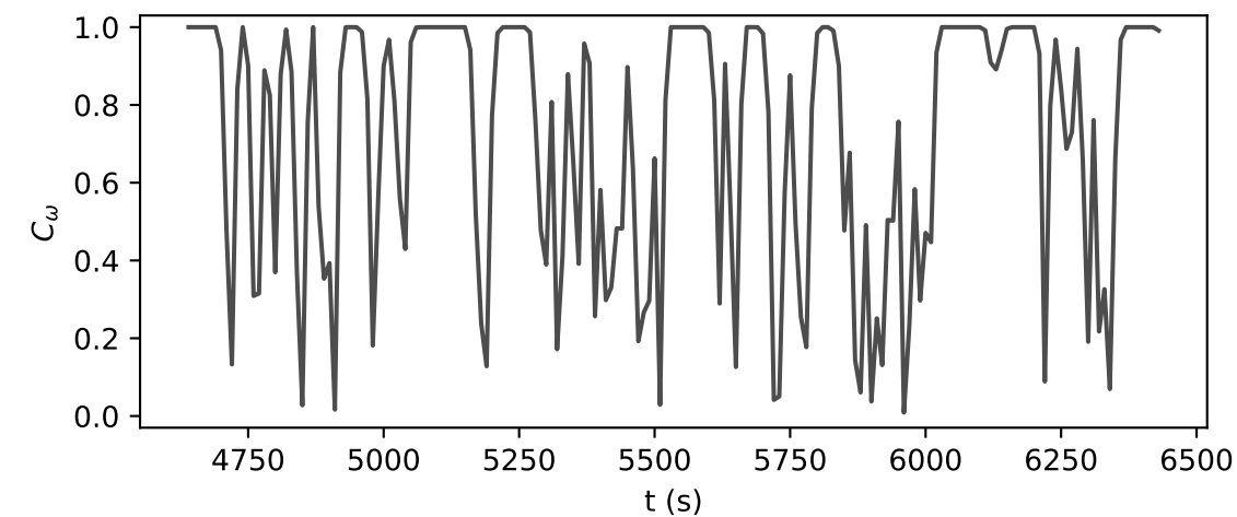
Turn-direction coherence
