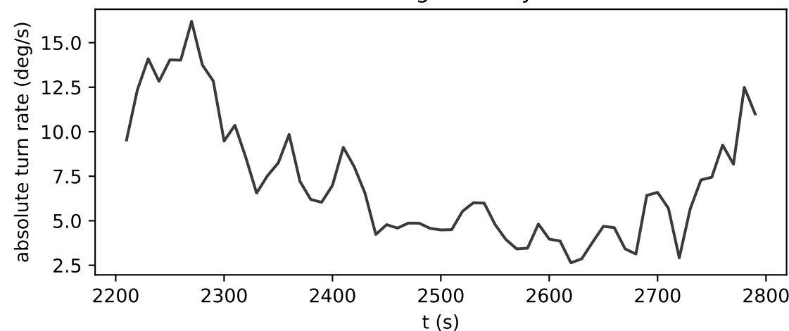
Turning intensity
