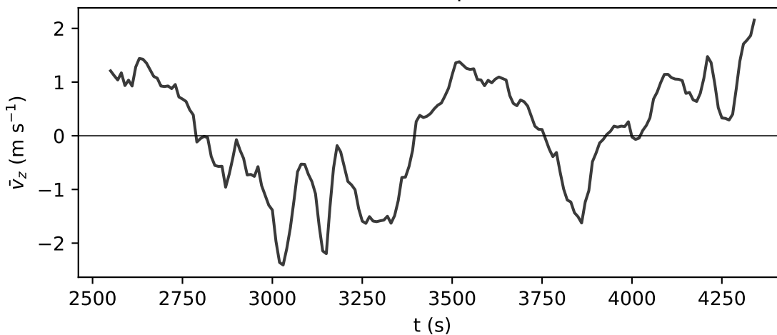
Turning intensity
