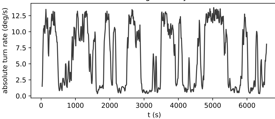
Turning intensity
