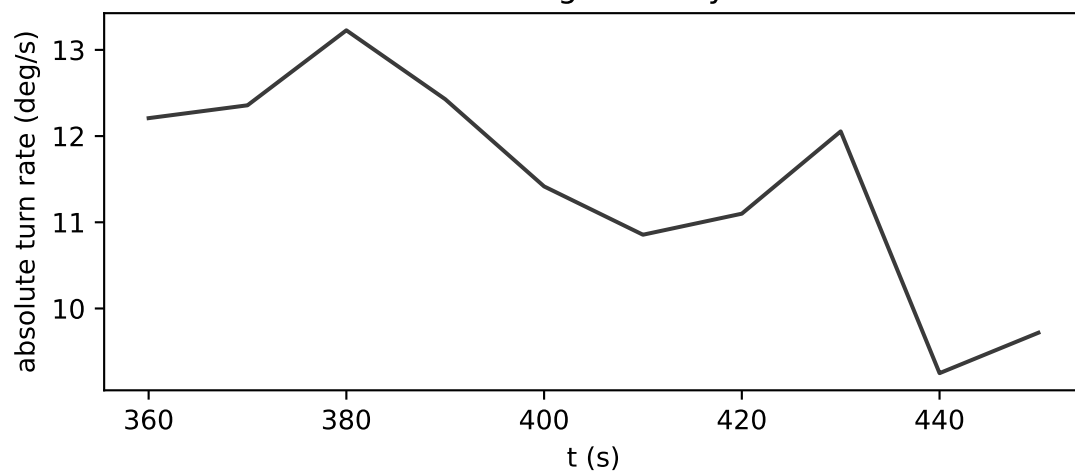
Turning intensity
