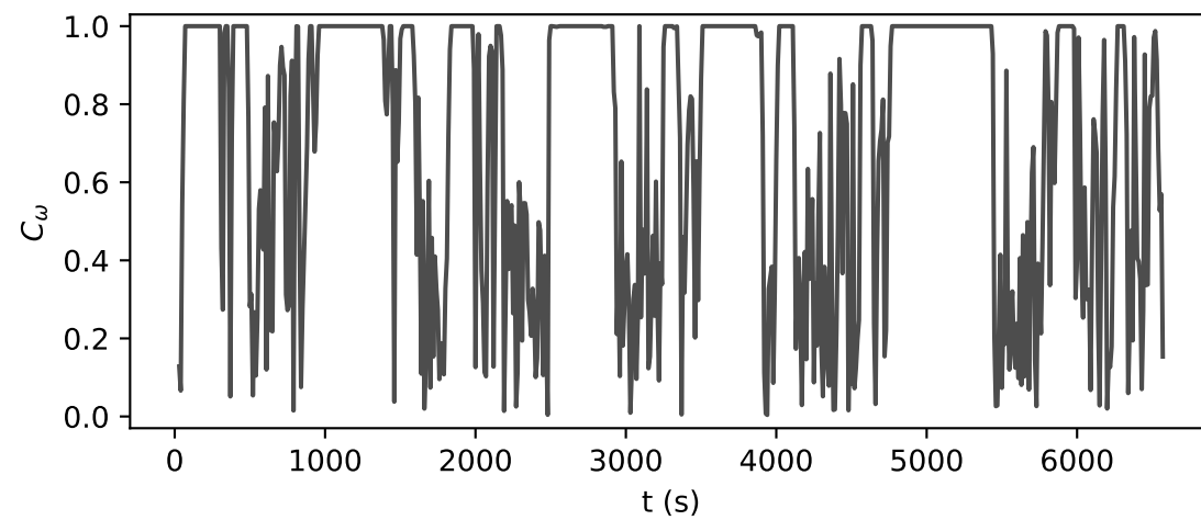
Turn-direction coherence
