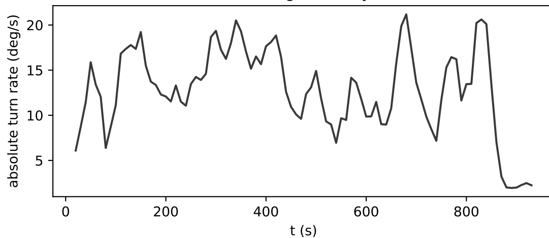
Turning intensity
