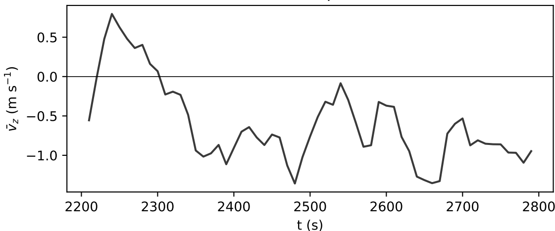
Turning intensity
