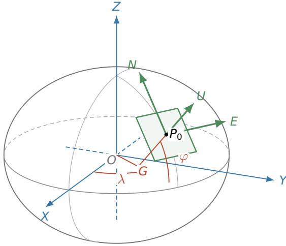
Figure 2.13. The ENU rotation: it turns a vector's global ECEF components into local East, North, Up ones. (a) The global ECEF frame ( X, Y, Z ) in blue, centred at the Earth's centre O ; the two red angles that locate the origin fix P_0 (the first fix of the trimmed track, Sec. 2.7.5): longitude \lambda , measured in the equatorial plane from the prime meridian, and geodetic latitude \varphi , the tilt of the ellipsoid normal, measured at the point G where the normal meets the equatorial plane; and the local ENU frame in green, tangent at P_0 . Flattening exaggerated as in Figure 2.12: U follows the normal G-P_0 , not the radius from O . The green arrows are the rows of the rotation matrix, as unit vectors. (b) Close-up of the tangent plane: a later fix's ECEF displacement \Delta\mathbf{X}(t) is the space diagonal of the box whose edges are its ENU components E(t) , N(t) , U(t) .
