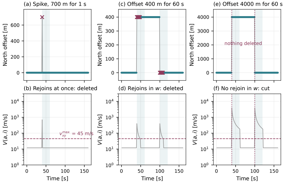
Figure 2.3. The three outcomes of the gate, obtained by running the implemented cleaning on constructed tracks. A paraglider cruises east at 12 \text{ m s}^{-1} at a 1 s cadence and is displaced north by 700 m for one fix (a), by 400 m for 60 s (c), and by 4,000 m for the same 60 s (e). Crosses mark the deleted fixes, dotted lines the segment boundaries, and the shaded band the span w a block may stay open, measured from its first fix. The lower row is the chord speed of Eq. (2.5), evaluated against the anchor the scan actually used, with the bound v_{xy}^{\max} dashed. A block closes where that curve falls back under the bound. In (c,d) the offset is below v_{xy}^{\max} w and is rejoined at both ends, so nine fixes go each time, among them good ones already back on the original route. In (e,f) nothing rejoins inside w : the displaced branch is kept whole and becomes its own segment. These are illustrative tracks, not archive data.
