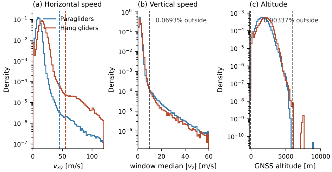
Figure 2.7. Fix-level cleaning: auditing the absolute bounds. Per-fix distributions of the quantities the absolute bounds test—bounds that serve both the out-of-range rule on the vertical channel and, through the v_{xy} bound, the impossibility gate that deletes an off-the-trend fix on the horizontal one (Sec. 2.7.2) – (a) horizontal speed v_{xy} , (b) the windowed GNSS med |v_z| of Eq. (2.7), the quantity the bound of Table 2.5 actually acts on, (c) GNSS altitude – pooled over a large paraglider subsample and the complete hang-glider population, with the adopted bounds dashed (Table 2.5); the y -axis is logarithmic so the sparse tail the bounds act on is visible. All x -axes are linear, so the distance from ordinary speeds to the threshold is directly readable. Panel (b) emphasizes the interval through 60 \text{ m s}^{-1} ; its exceedance annotation includes the full sample. The x -axis of panel (c) is extended to 10,000 \text{ m} regardless of the sample or the bound. Panel (a) spans 0 \text{ m s}^{-1} to 120 \text{ m s}^{-1} . Histogram densities use the full finite-sample denominator; the displayed tail is not renormalized. Binning choices and sample sizes: paragraph Diagnostic sample of Sec. 2.7.2 (p. 14). This figure audits the absolute bounds only; the Hampel and frozen-lock detectors have no per-fix distribution to read a threshold off, and require the example inspection and sensitivity assessment described below. The annotated fractions count bound exceedances, not fixes actually removed: deletion also depends on the rejoin rule and vertical invalidation on neighbouring windows.
