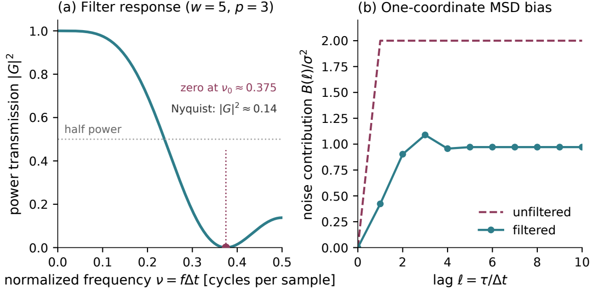
Figure 2.19. Exact effects of the five-sample cubic filter away from segment edges. Left: power transmission |G|^2 of Eq. (2.29) against the normalized frequency \nu = f\Delta t of Eq. (2.28), in cycles per sample. The axis is cadence free, and \nu = 0.5 is the Nyquist frequency 1/(2\Delta t) , which is 0.5 Hz at a 1 s cadence and 0.1 Hz at a 5 s one. Half the power survives near \nu \approx 0.24 , the response vanishes at \nu_0 \approx 0.375 , and the sidelobe beyond it still transmits |G|^2 \approx 0.14 at Nyquist. Right: additive one-coordinate MSD from independent unit-variance measurement noise. The remaining bias depends on lag and does not equal the unfiltered 2\sigma^2 .
