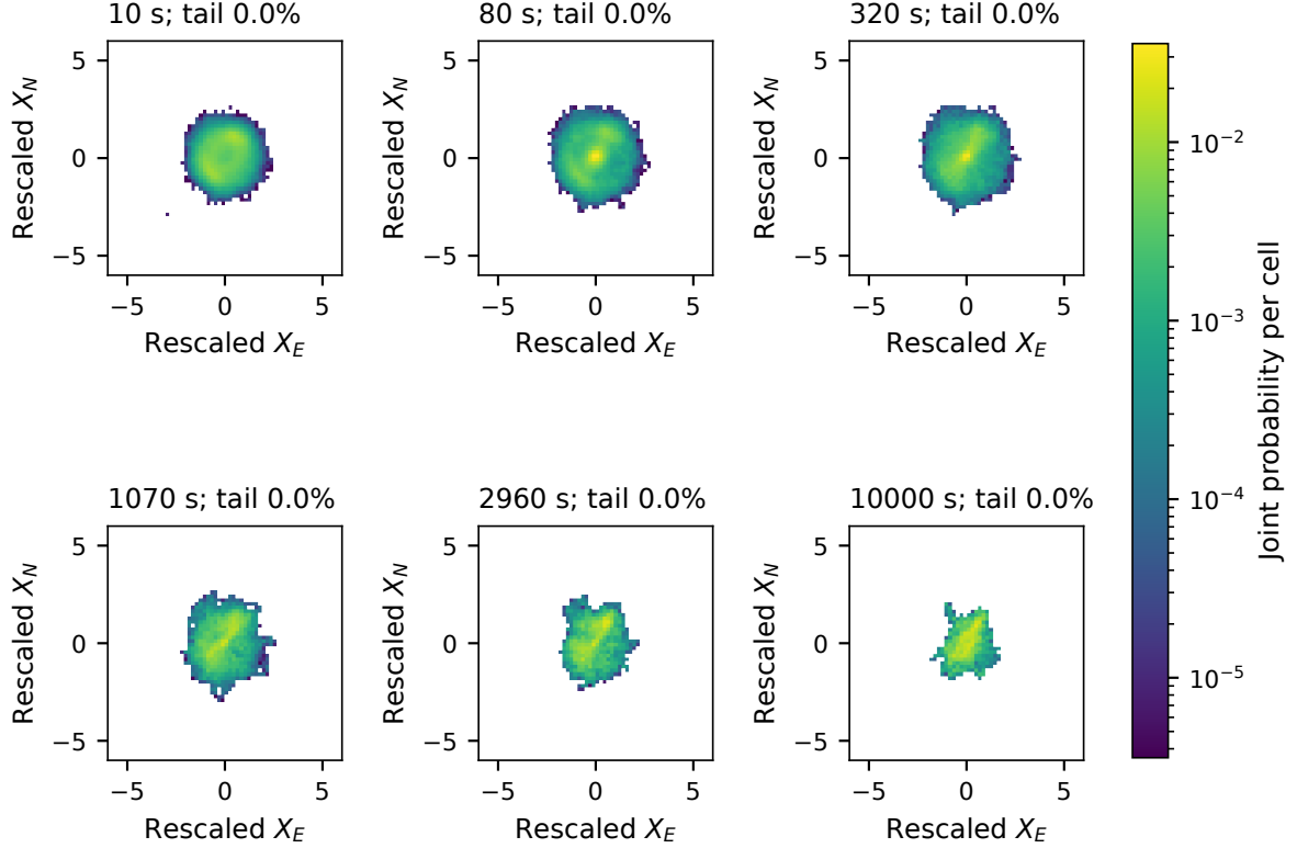
Figure 3.13. Signed joint displacement laws for the fixed paraglider population, after one scalar power rescaling of both axes. Colours show probability per common cell. Each panel reports the mass outside the displayed square; overflow cells are retained in numerical comparisons. These are descriptive distributions, not iid hypothesis tests.
