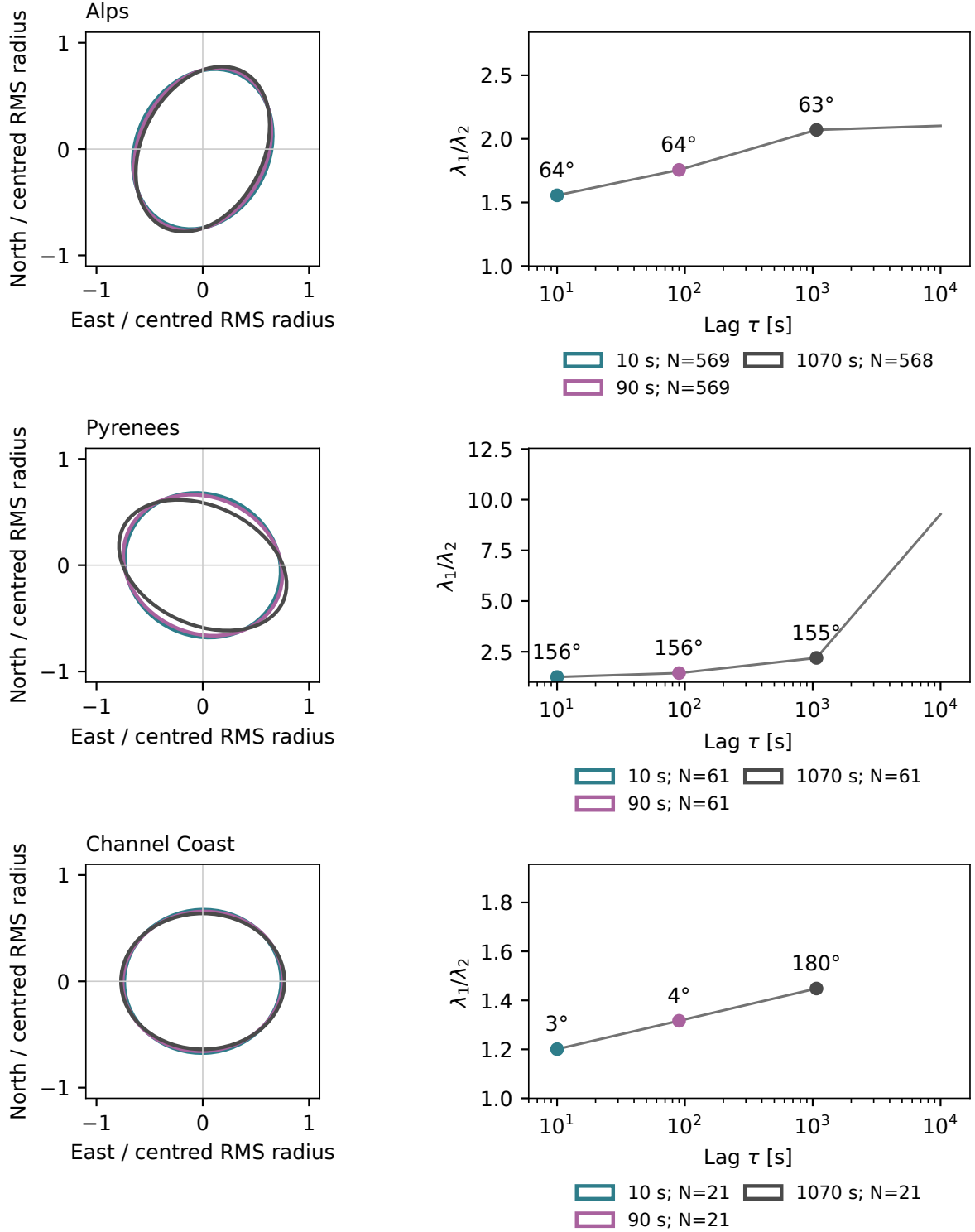
Figure 3.15. Regional principal-axis diagnostics in the paraglider eligible archive. Covariances are centred before diagonalisation. The principal direction is an axis modulo 180^\circ and its interpretation depends on the separation of the two eigenvalues. Region counts and lag dependence delimit the evidence. These measurements describe displacement geometry and do not identify wind.
