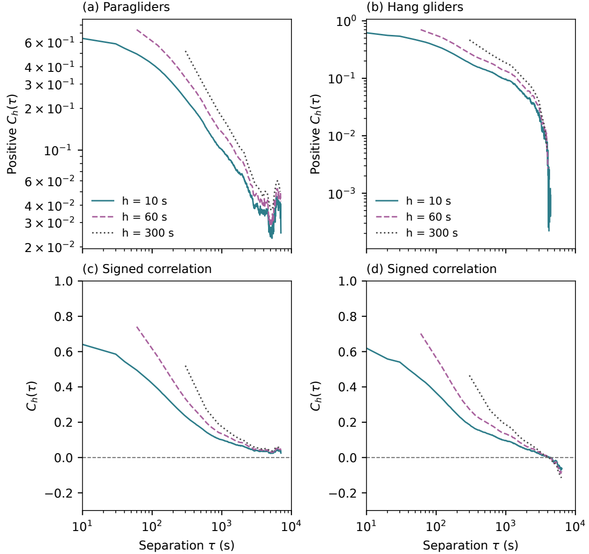
Figure 3.20. Velocity memory at averaging widths h = 10, 60 and 300 s. The upper panels use log–log axes for positive correlations; nonpositive values interrupt the curves. The lower panels show the same estimates with a linear vertical axis, preserving zero crossings and anticorrelation. At least 20 contributing flights are required, with separation no shorter than h and no longer than one quarter of each contributing velocity record. A visually straight part of the upper curves is a possible scaling interval, not evidence of an asymptotic law.
