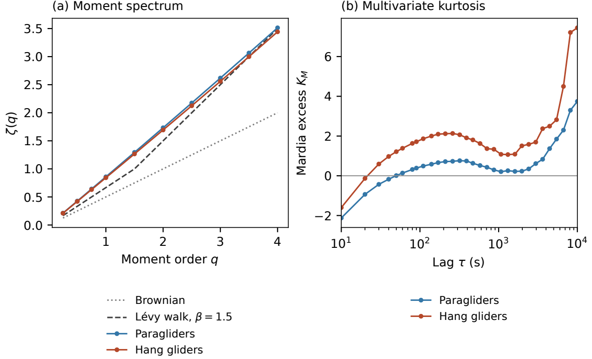
Figure 3.19. Displacement moment spectra and centred multivariate kurtosis in the diagnostic eligible archive, with theoretical moment spectra shown as reference curves. These observables constrain the growth and shape of the increment distribution, respectively, but neither alone identifies the generating process.
