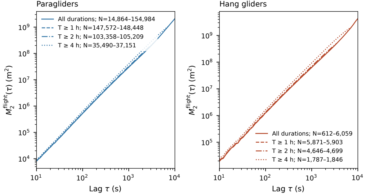
Figure 3.21. Time-averaged squared displacement by retained flight duration. Cohorts are nested; legend counts give the range of contributing flights. Each lag requires at least 30 flights. Threshold curves end at T_0/2 , while the all-duration curve extends to 10,000 s. Shorter flights progressively leave the reference near T_0/2 , bringing the populations closer by selection.
