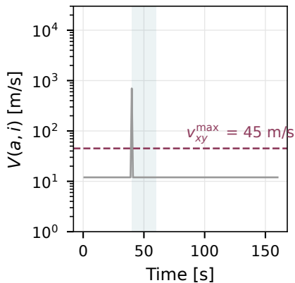
(b) Rejoins at once: deleted
