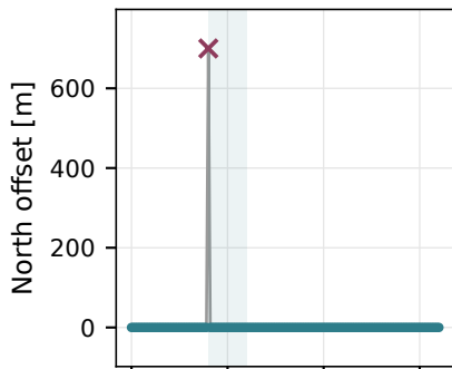
(b) Rejoins at once: deleted
