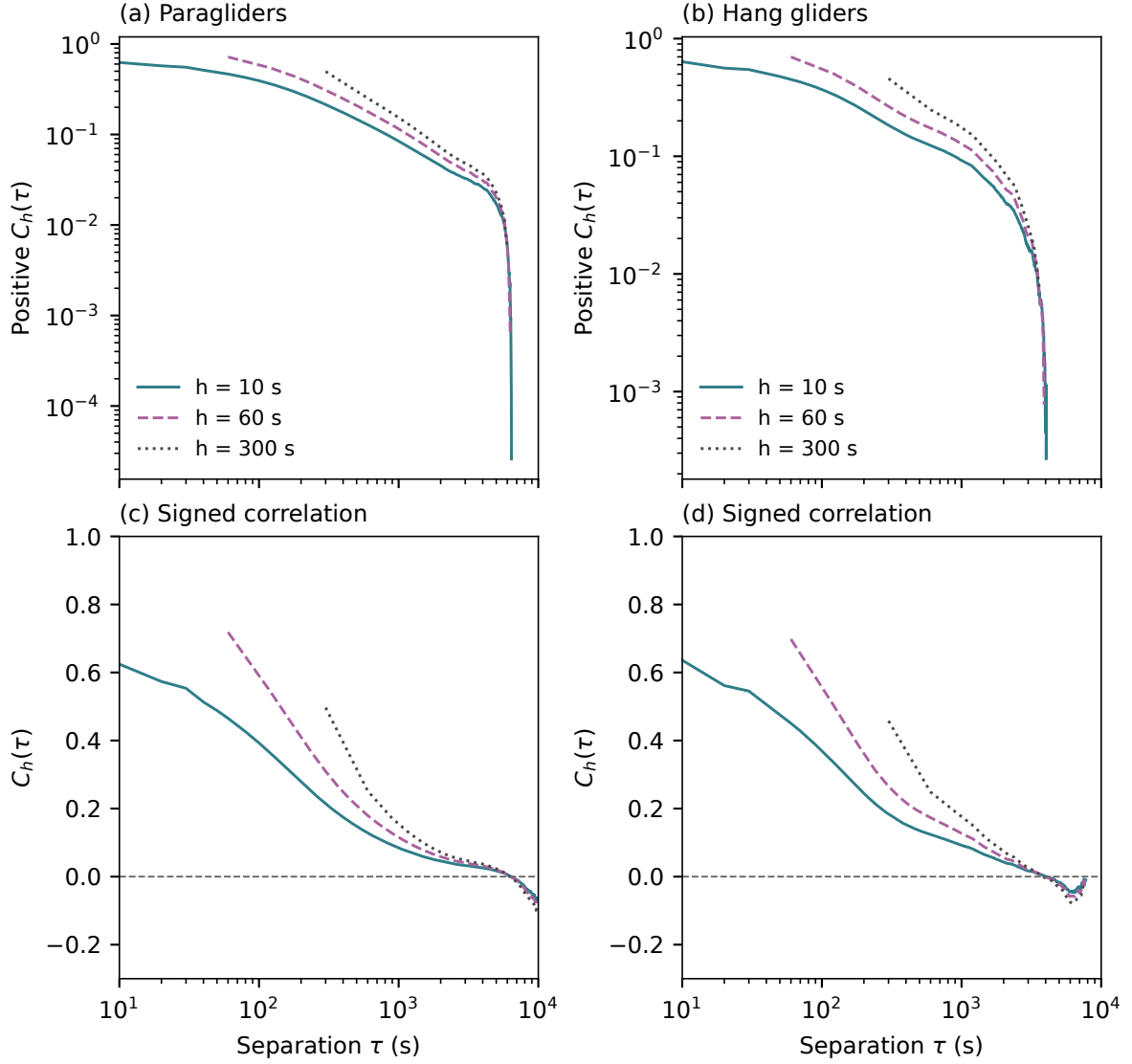
Figure 3.24. Velocity memory at averaging widths h = 10, 60 and 300 s. The upper panels use log-log axes for positive correlations; nonpositive values interrupt the curves. The lower panels show the same estimates with a linear vertical axis, preserving zero crossings and anticorrelation. At least 20 contributing flights are required, with separation no shorter than h and no longer than one quarter of each contributing velocity record. A visually straight part of the upper curves is a possible scaling interval, not evidence of an asymptotic law.
