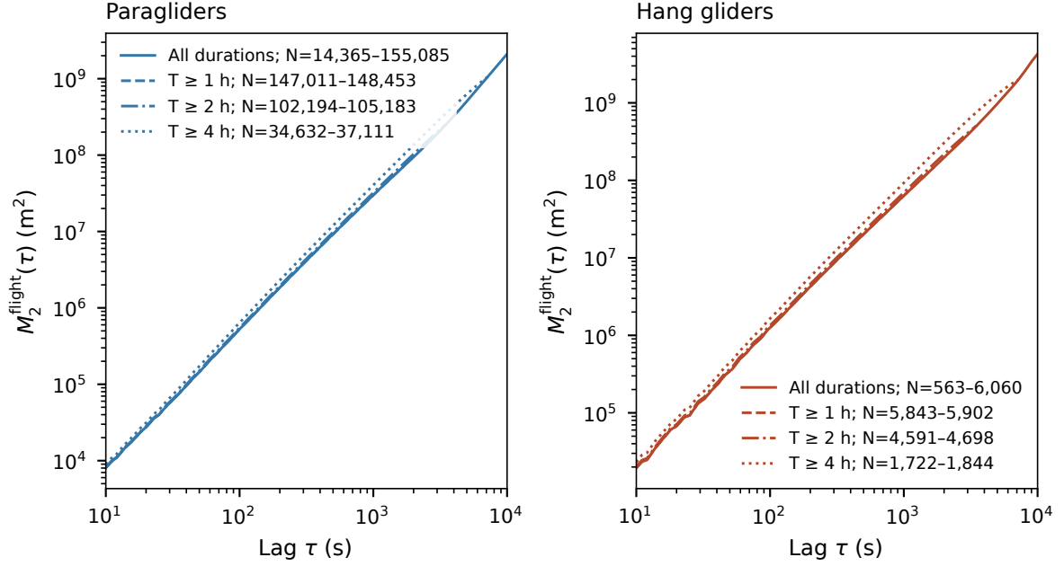
Figure 3.19. Time-averaged squared displacement by retained flight duration. Cohorts are nested; legend counts give the range of contributing flights. Each lag requires at least 30 flights. Threshold curves end at T_0/2 , while the all-duration curve extends to 10,000 s. Shorter flights progressively leave the reference near T_0/2 , bringing the populations closer by selection.
