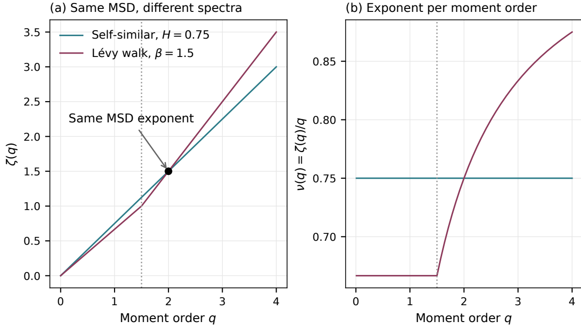
Figure 3.22. Theoretical comparison. A self-similar process with H = 0.75 and a standard Lévy walk with \beta = 1.5 have the same MSD exponent, \zeta(2) = 1.5 , but different moment spectra. The dashed vertical line marks q = \beta . These are asymptotic predictions, not simulated or empirical estimates.
