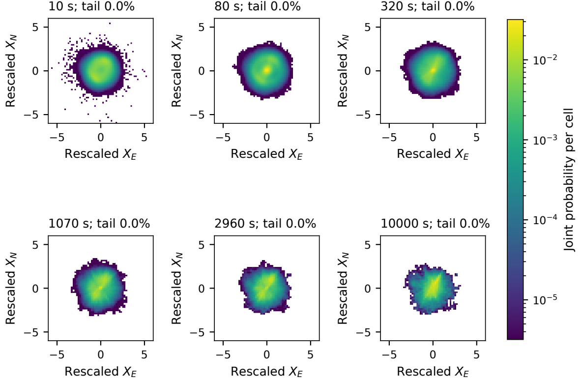
Figure 3.12. Signed joint displacement laws for the fixed paraglider population, after one scalar power rescaling of both axes. Colours show probability per common cell. Each panel reports the mass outside the displayed square; overflow cells are retained in numerical comparisons. These are descriptive distributions, not iid hypothesis tests.
