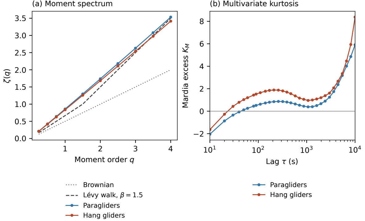
Figure 3.23. Displacement moment spectra and centred multivariate kurtosis in the diagnostic eligible archive, with theoretical moment spectra shown as reference curves. These observables constrain the growth and shape of the increment distribution, respectively, but neither alone identifies the generating process.
