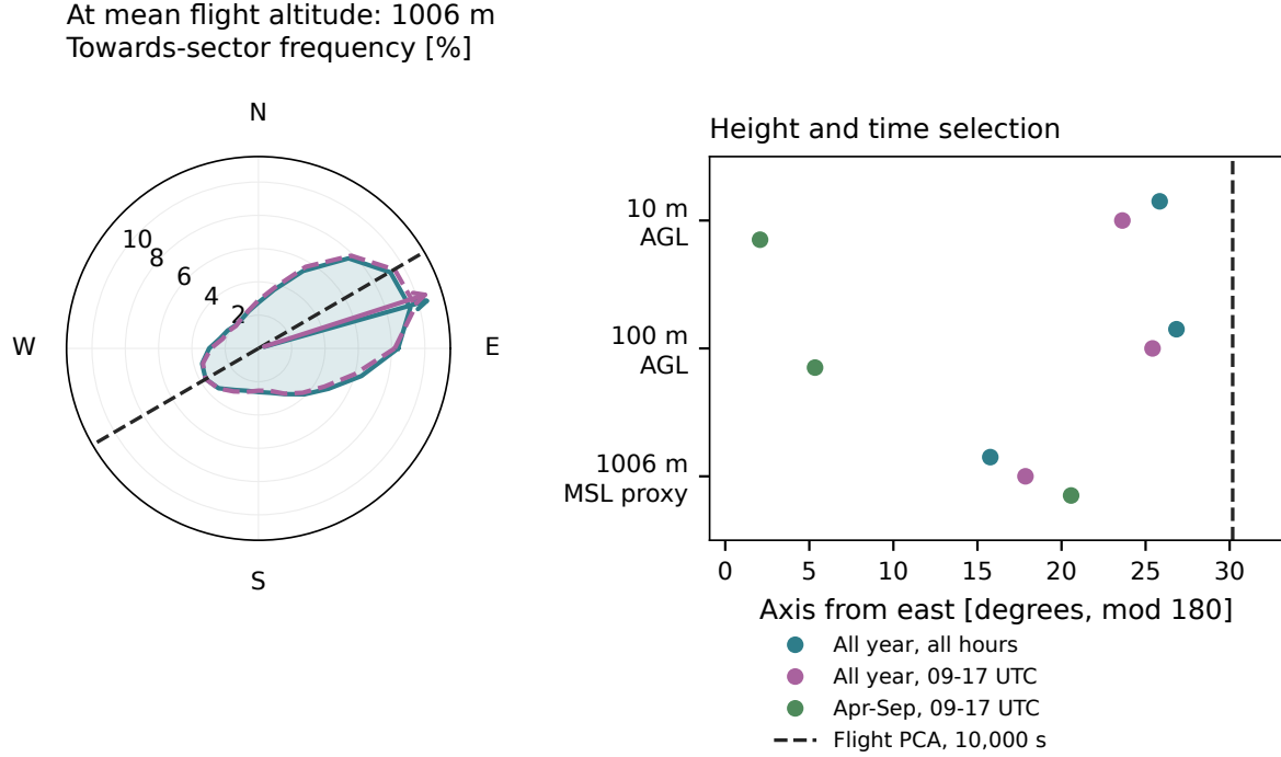
Figure 3.23. ERA5 wind at mean coastal flight altitude and the paraglider PCA at 10,000s. Left: frequencies of air motion towards 15-degree sectors at 1,006 m, for all-year all hours and all-year 09–17 UTC. Speeds below 0.5 \text{ m s}^{-1} are excluded only from the frequency curves; arrows show the vector means using all selected hours. Right: wind axes at flight altitude, approximately above mean sea level, and at 10 and 100 m above ground (AGL). The warm daytime selection is shown as a separate check. The dashed black line is the same flight covariance axis in every comparison.
