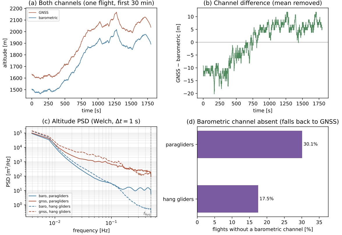
Figure 4.1: Barometric vs GNSS altitude noise. For one representative flight (the one with the most fixes in the subsample), over its first 30 min: (a) the two raw channels overlaid – they track the same climb, but the GNSS trace is visibly noisier; (b) their difference GNSS–barometric (mean removed), which isolates that noise. Over the ensemble: (c) mean Welch power spectra of the two channels, per discipline (Appendix B); the dotted line is the Nyquist frequency f_{\text{Nyq}} = 1/(2\Delta t) , the highest frequency the sampling can resolve. It is a single line because the pooled flights are all resampled to the same modal \Delta t before averaging, so they share one \Delta t – hence one f_{\text{Nyq}} . (d) Fraction of flights whose barometric channel is absent, per discipline; see the main text for how these were measured and their precision.
