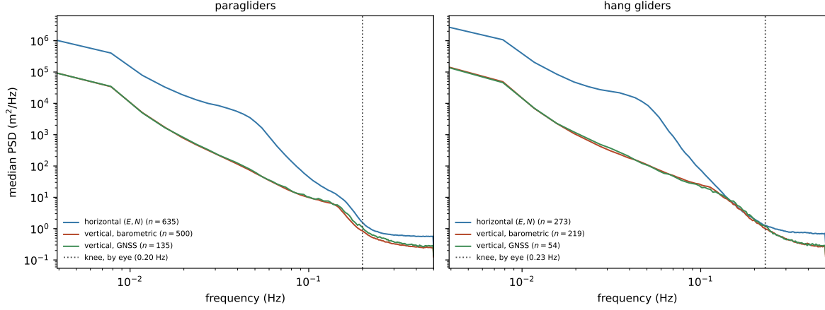
Figure 2.9. The ensemble Welch power spectral density of each channel, by discipline: horizontal ( E , N pooled), barometric-vertical and GNSS-vertical. Median over a seeded sample of up to 900 flights per discipline, restricted to those within 0.25 s of the dominant 1 Hz cadence so every spectrum shares one frequency grid; the usable count per channel is in its legend entry. The dotted line is the knee frequency read by eye off the curves, not fitted: 0.20 Hz for paragliders, 0.23 Hz for hang gliders. Within a panel the three channels flatten into the same floor at visibly the same frequency; paragliders and hang gliders fly at very different speeds, yet the two panels’ knees still land within a few hundredths of a hertz of each other, the cross-check the main text draws on.
