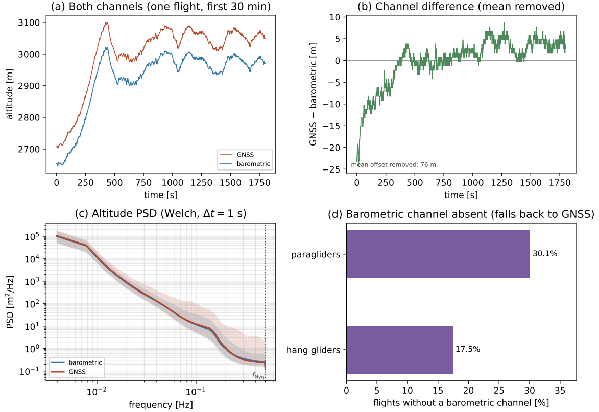
Figure 3.1: Barometric vs GNSS altitude noise. Panels (a)/(b): one representative flight over a 30 min window. (a) the two raw channels on a single shared axis, so their offset – the gap between the pressure and ellipsoidal references, tens of metres – is read directly, while both track the same vertical motion. (b) their difference GNSS–barometric (mean removed, not detrended): the offset drifts by tens of metres over the flight, a real feature – plausibly the barometric channel’s slow departure from the ICAO standard atmosphere as altitude changes – not noise, so only its constant part (annotated) is subtracted. Panels (c)/(d): over the ensemble. (c) the per-frequency median Welch spectrum of each channel (Appendix B), pooled over the two disciplines (whose spectra coincide), with a shaded 10 to 90 percentile band across flights. The median lines nearly coincide: for the typical flight the two channels are comparable at high frequency, both near the floor set by the shared metre-resolution logging. The bands carry the real story – the barometric band stays tight (uniformly clean), whereas the GNSS band fans out by one to two orders of magnitude towards Nyquist, driven by a minority of flights with heavy multipath noise. The median, not the mean, precisely because these per-flight spectra are heavy-tailed and a mean is dominated by that noisy minority (Sec. 3.5.1). The dotted line is the Nyquist frequency f_{\text{Nyq}} = 1/(2\Delta t) . (d) Fraction of flights whose barometric channel is absent, per discipline. (implementation details: Sec. 3.5.1)
