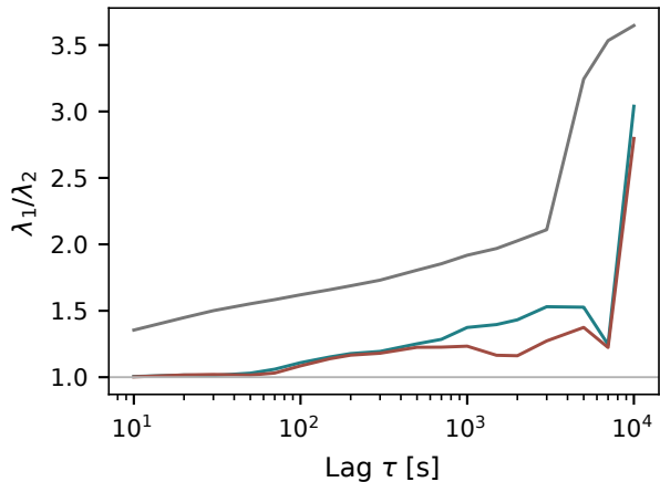
Centred covariance anisotropy
