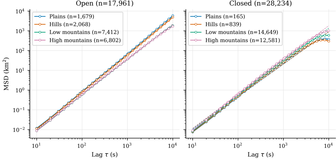
Figure 3.6. Paraglider transport by declared circuit and initial altitude, with fixed flights and segments throughout 10–10000 s. Markers give MSD estimates, shaded bands their pointwise 90% intervals, and dashed lines the global log–log fits. The identical axes permit comparison of displacement amplitude and growth rate.
