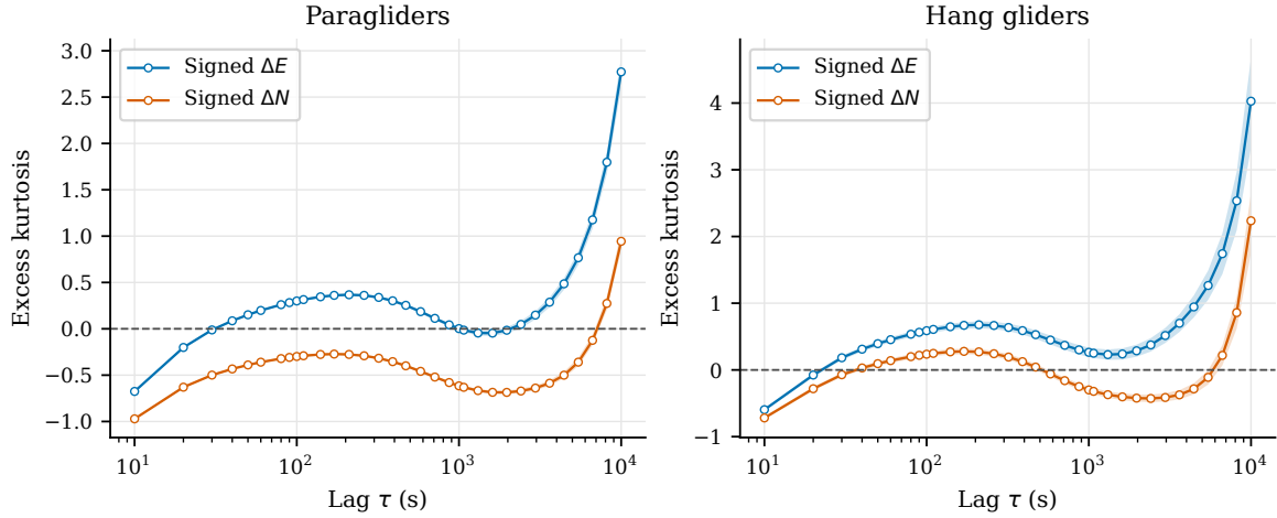
Figure 3.12. Signed-component Fisher excess kurtosis at the same lags, with the same flights, segments and weights as the quantiles and moments. The dashed line is the Gaussian marginal reference. Bands use the coupled cluster bootstrap.
