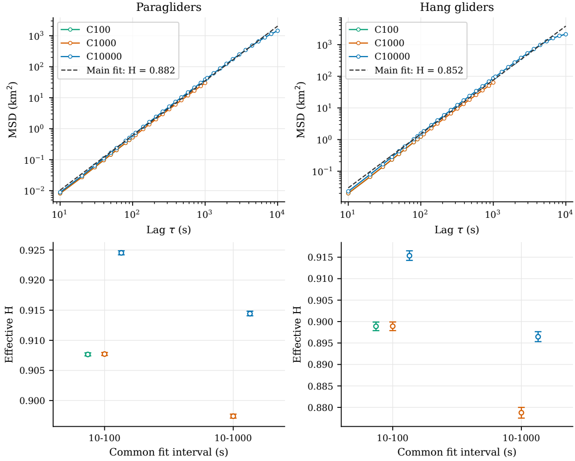
Figure 3.5. Effect of duration selection. Top: MSD in the three nested cohorts; dashed lines fit the main cohort over 10–10000 s. Bottom: effective H with 90% intervals, fitted over 10–100 s for all three cohorts and 10–1000 s for the two longer cohorts. Fits within each comparison use identical lag values.
