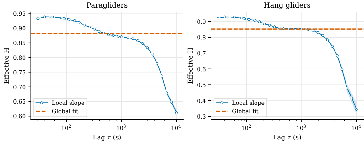
Figure 3.10. Local and global effective MSD exponents on the fixed main cohort. Bands are pointwise 90% bootstrap intervals. The global fit compresses the full curve into one number; the local slopes expose its scale dependence.
