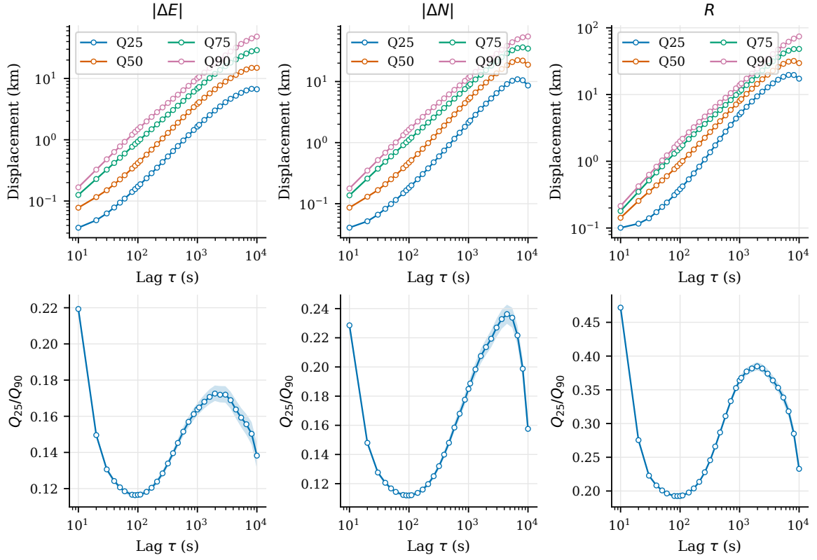
Figure 3.8. The same amplitude quantiles and ratio for hang gliders, with an independent main cohort and the same sampling convention.
