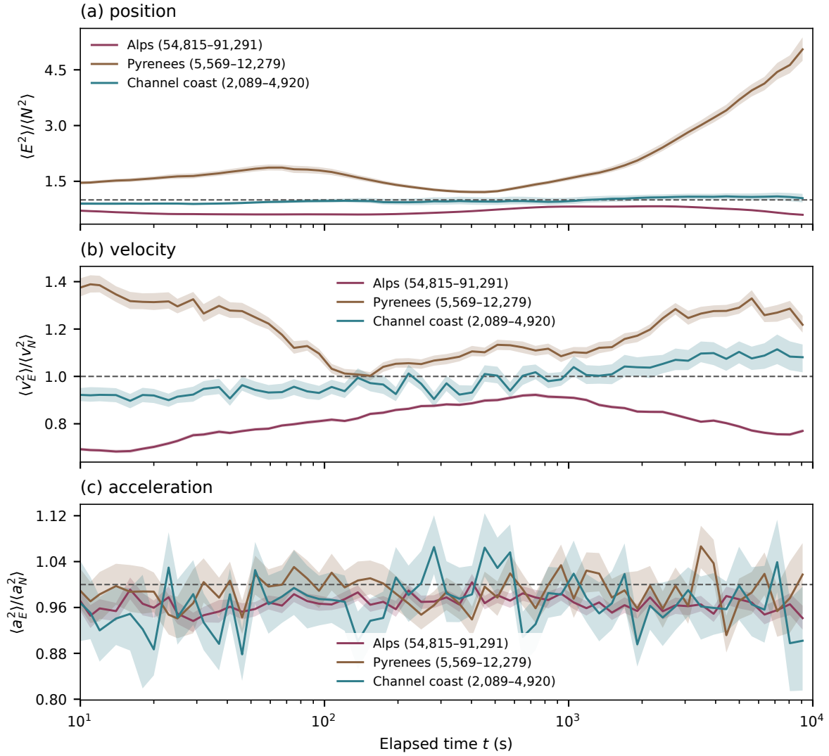
Figure 3.25. Paraglider east/north second-moment ratios by take-off region, against time since launch. Position, velocity and acceleration all retain mean motion. Shading gives pointwise 10–90% site-day bootstrap ranges; times require 30 flights and 10 clusters, with flight-count ranges in the legends. Missing site/date records form singleton groups. Unity marks equal component moments, leaving cross moments and angular structure untested. Panel limits follow each quantity; no scaling exponent is fitted.
