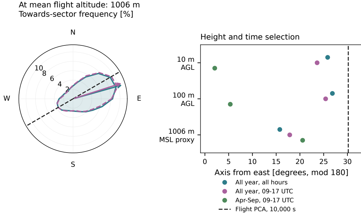
Figure 3.24. ERA5 wind at mean coastal flight altitude and the paraglider PCA at 10,000s. Left: frequencies of air motion towards 15-degree sectors at 1,006 m, for all-year all hours and all-year 09–17 UTC. Speeds below 0.5 \text{ m s}^{-1} are excluded only from the frequency curves; arrows show the vector means using all selected hours. Right: wind axes at flight altitude, approximately above mean sea level, and at 10 and 100 m above ground (AGL). The warm daytime selection is shown as a separate check. The dashed black line is the same flight covariance axis in every comparison.
