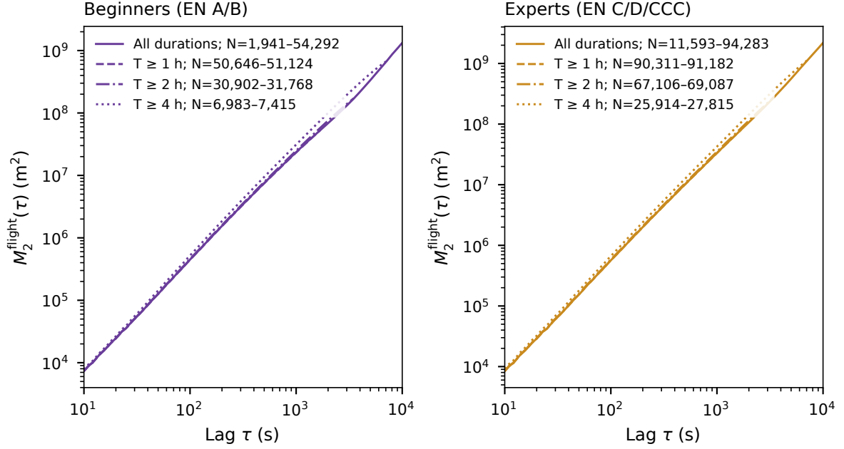
Figure 3.35. The duration comparison repeated for beginners (EN A/B) and experts (EN C/D/CCC), using the same estimator, lag limits and minimum support as Fig. 3.34. Counts refer to distinct flights, and overlapping groups do not constitute independent samples. Tandem, non-certified and unknown equipment is omitted from this contrast.
