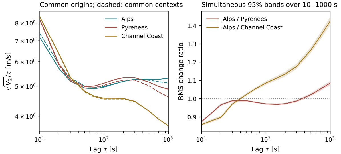
Figure 3.30. Paraglider population controls. Left: common-origin curves, with the common-context standardisation dashed. The dashed curves are descriptive point estimates. Right: regional ratios of the unstandardised common-origin curves; shading is simultaneous over the 18-lag grid's supported subset through 1000 s. These controls do not match meteorology, local terrain exposure or pilot identity.
