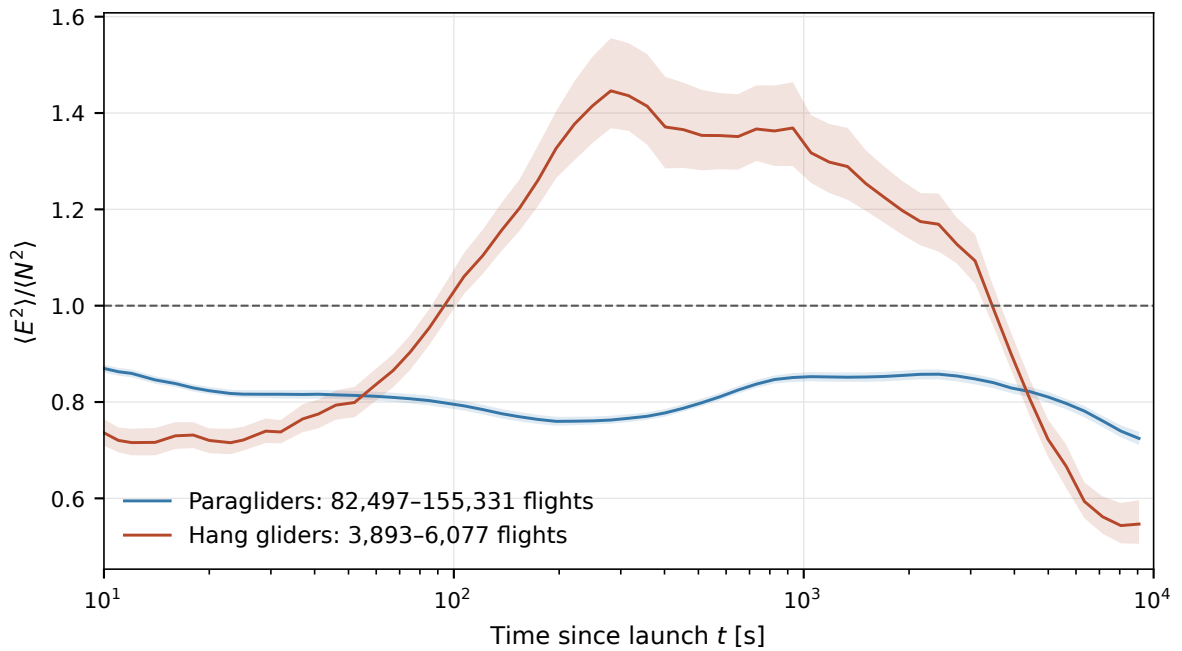
Figure 3.21. Archive east–north second-moment ratio against elapsed time since launch. Curves show the observed ratio; shading gives the pointwise 10–90% range from 200 bootstrap resamples of whole take-off-site-and-day groups. Only times with at least 30 paired flights and 10 contributing clusters are shown; legend counts give the minimum and maximum flight support along each curve. These are display minima, not a precision criterion. Unity is a necessary condition for isotropy, not sufficient evidence of it; these bands are not a simultaneous confidence statement across all times.
