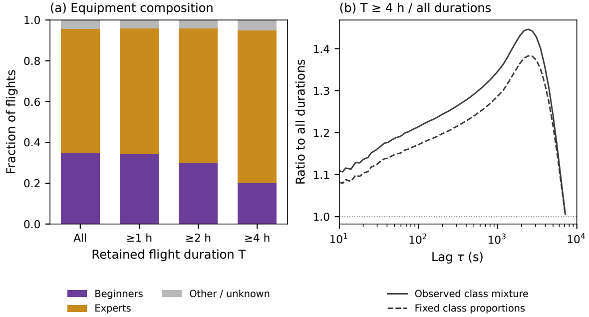
Figure 3.36. Equipment composition and its contribution to the duration comparison. Left: proportions of flights in the nested duration cohorts, including other or unknown equipment (6,510 flights in the full eligible sample). Right: the four-hour/all-duration MSD ratio among known classes, using the observed lag-dependent mixture or fixed class weights. Unity denotes equal MSD amplitudes at that lag, not equal trajectories or established statistical independence.
