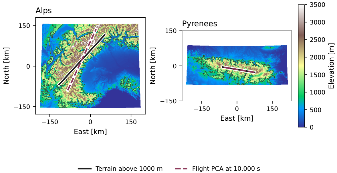
Figure 3.23. Independent terrain orientation compared with the paraglider displacement covariance at 10,000 s. Elevation and the 1,000 m contour come from ETOPO 2022 [28]. The solid dark line is the highland-footprint axis; the dashed coloured line is the flight PCA axis, translated to the same centre for comparison. Line lengths carry no displacement or ridge-length information. Map coordinates are kilometres east and north of each box centre.
