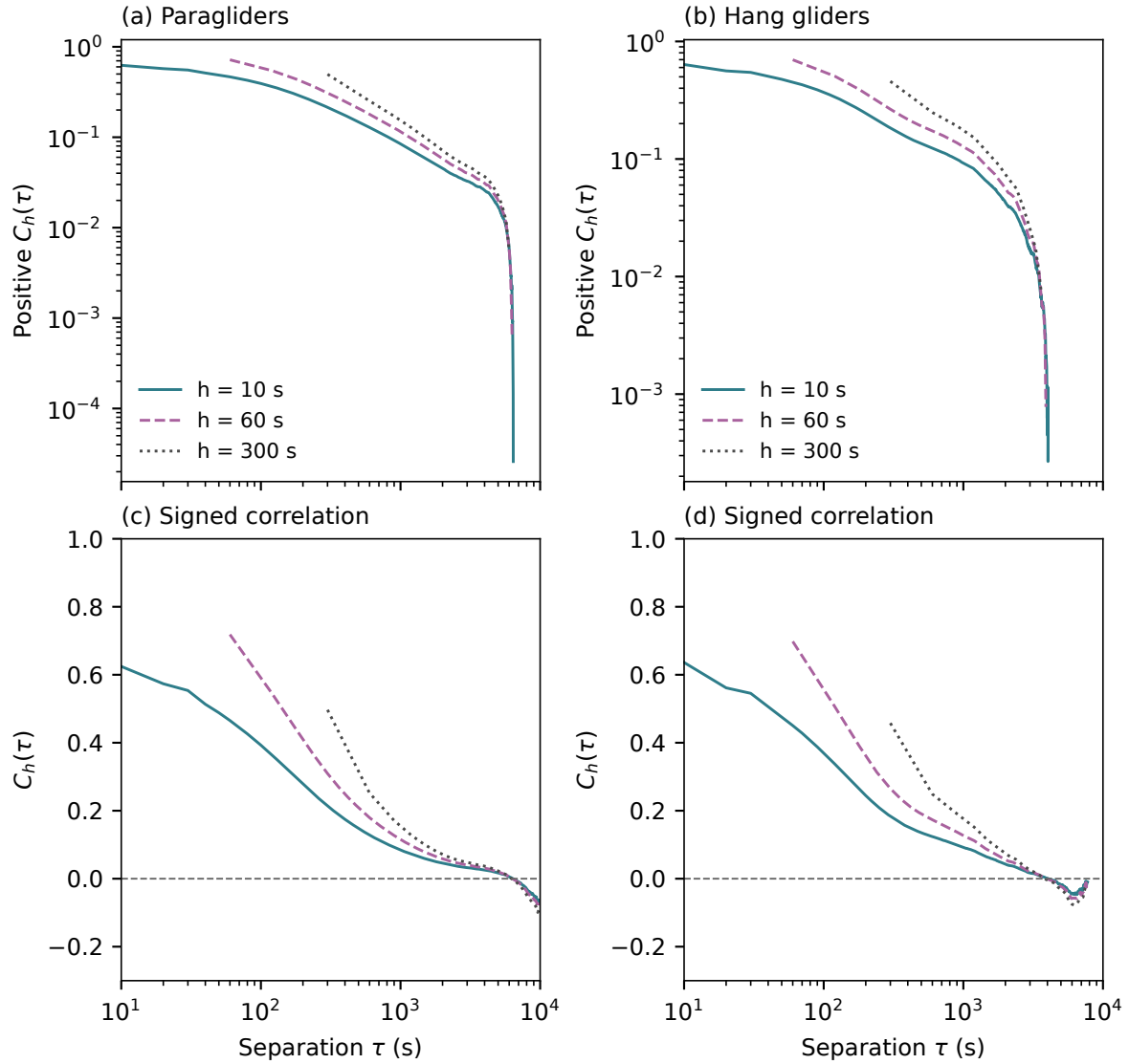
Figure 3.39. Velocity memory at averaging widths h = 10, 60 and 300 s. The upper panels use log-log axes for positive correlations; nonpositive values interrupt the curves. The lower panels show the same estimates with a linear vertical axis, preserving zero crossings and anticorrelation. At least 20 contributing flights are required, with separation no shorter than h and no longer than one quarter of each contributing velocity record. A visually straight part of the upper curves is a possible scaling interval, not evidence of an asymptotic law.
