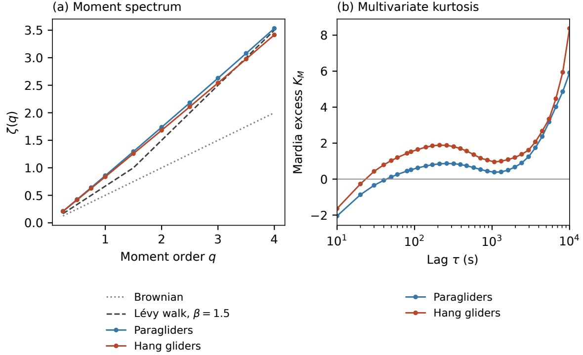
Figure 3.38. Displacement moment spectra and centred multivariate kurtosis in the diagnostic eligible archive, with theoretical moment spectra shown as reference curves. These observables constrain the growth and shape of the increment distribution, respectively, but neither alone identifies the generating process.
