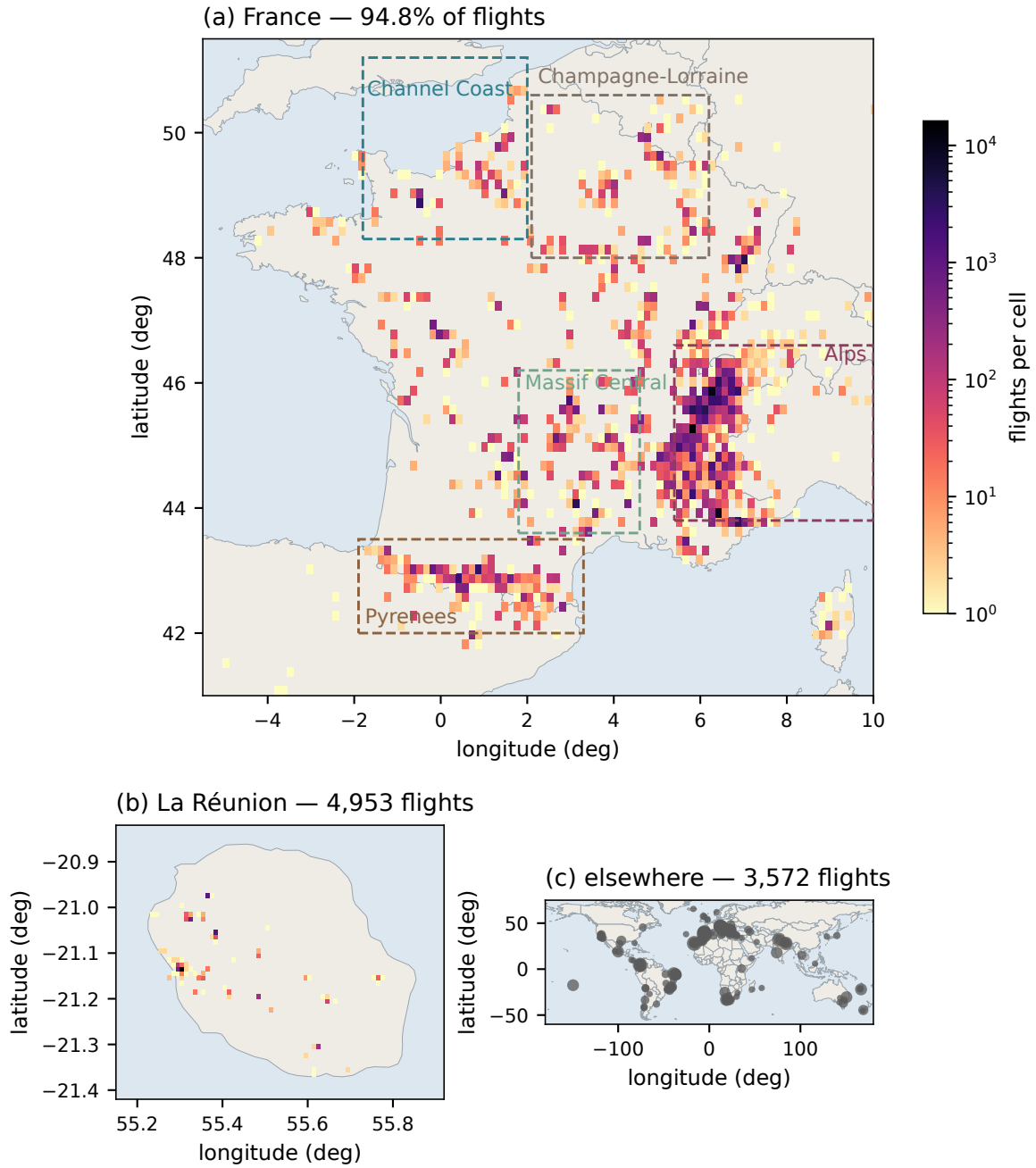
Figure 2.23. Take-off sites of the retained ensemble, on three frames, pooling both disciplines throughout. (a) Metropolitan France, density on a 0.15^\circ cell; the dashed boxes mark the geographic windows in Table 2.9, including Champagne-Lorraine; no altitude preselection is applied to this map. (b) La Réunion, on a 0.01^\circ cell, the one overseas department with a substantial share. (c) Everything else, one marker per 0.5^\circ cell with the area set by its count.
