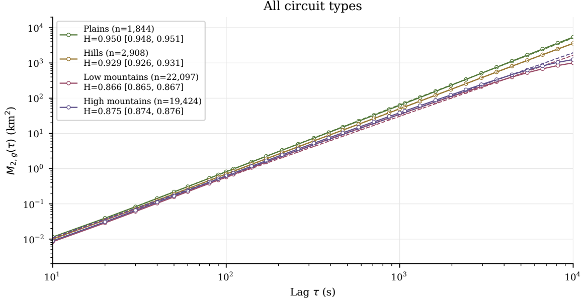
Figure 3.8. Paraglider MSD by initial altitude, pooling circuit types and equipment classes. The four groups partition the fixed cohort. The altitude thresholds describe the initial cleaned fix, rather than the relief along the trajectory.
