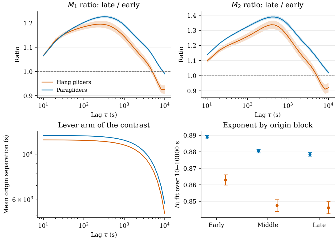
Figure 3.19. Origin dependence of the increment law in the main cohort. Top: the ratio of the late-block to the early-block radial moments, with 95% paired bootstrap bands and the stationary-increment value as a dashed line. Bottom left: the mean separation between the two blocks of origins, which shrinks as the lag consumes the segment. Bottom right: H fitted in each block over 10–10000 s. Bands and bars are pointwise.
