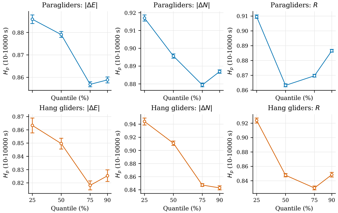
Figure 3.15. Global quantile exponents from 10–10000 s fits. Error bars are the 5th–95th percentiles of the refitted bootstrap slopes. A common scale exponent would give a horizontal sequence within each panel.
