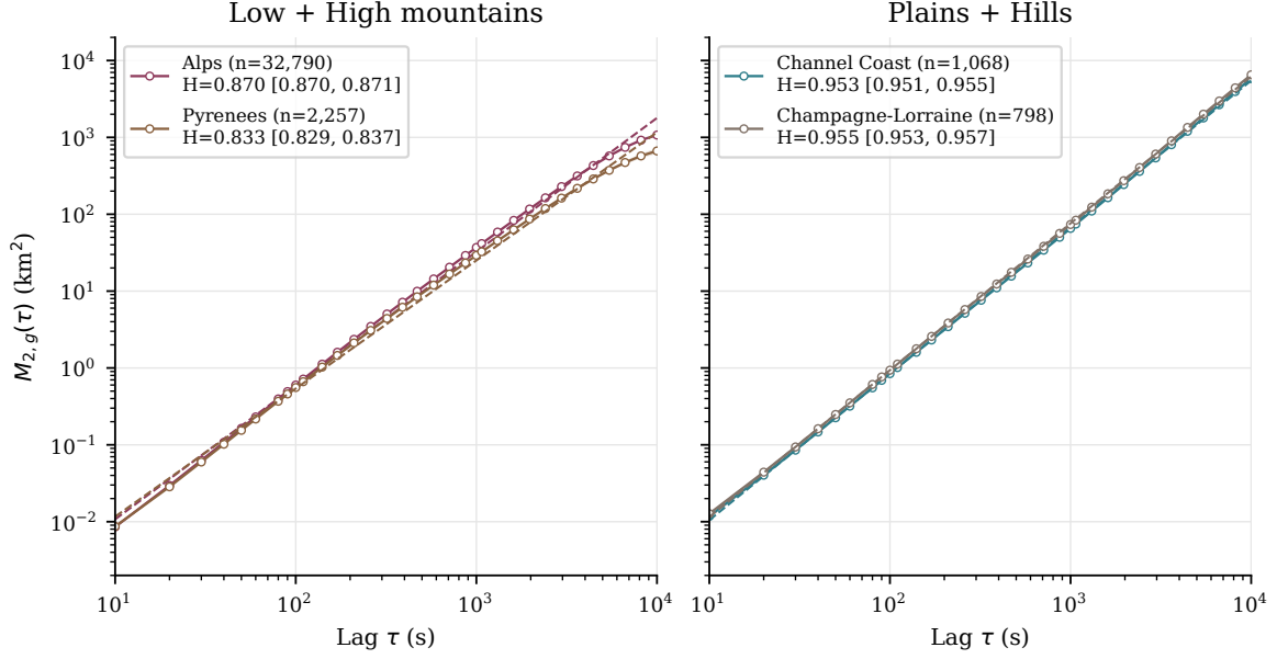
Figure 3.9. Regional paraglider MSDs. Left: Alps and Pyrenees. Right: Channel Coast and Champagne-Lorraine. The left panel retains only Low/High mountains within each box; the right retains only Plains/Hills. Circuit types and equipment classes are pooled. Counts and fits refer to the preselected populations; both panels share the same axes.
