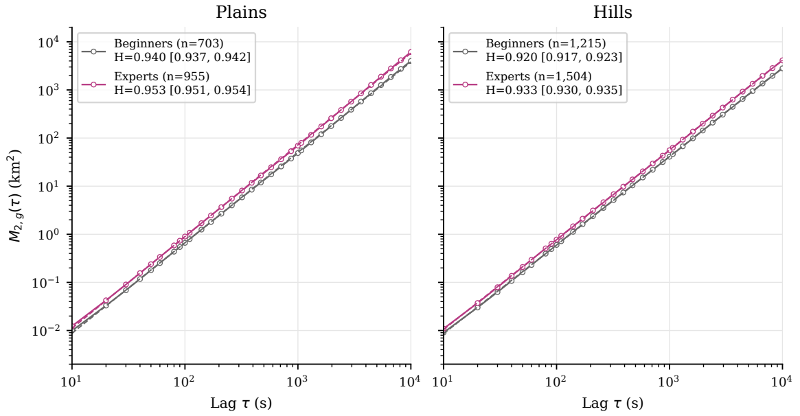
Figure 3.12. Beginners and experts within Plains and Hills, shown separately. Estimator, fit range, axes and uncertainty convention are the same as in Figure 3.11.
