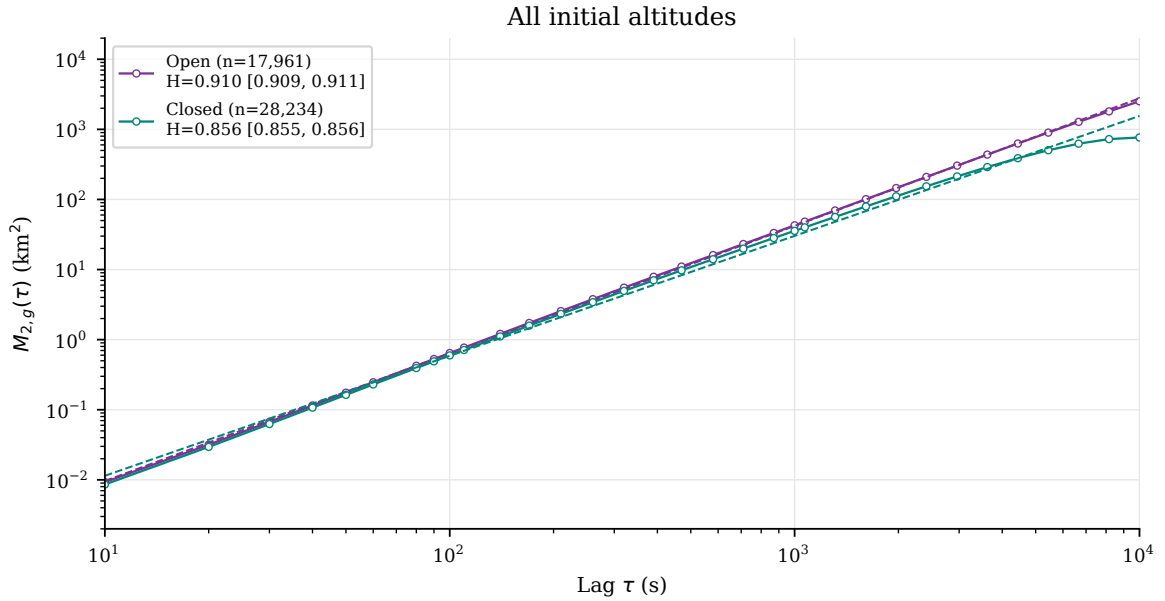
Figure 3.6. Paraglider MSD by declared circuit, pooling initial altitudes. Solid curves join the equal-flight estimates; dashed lines are fits over 10–10000 s. Counts, effective exponents and 90% intervals refer to the fixed groups.
