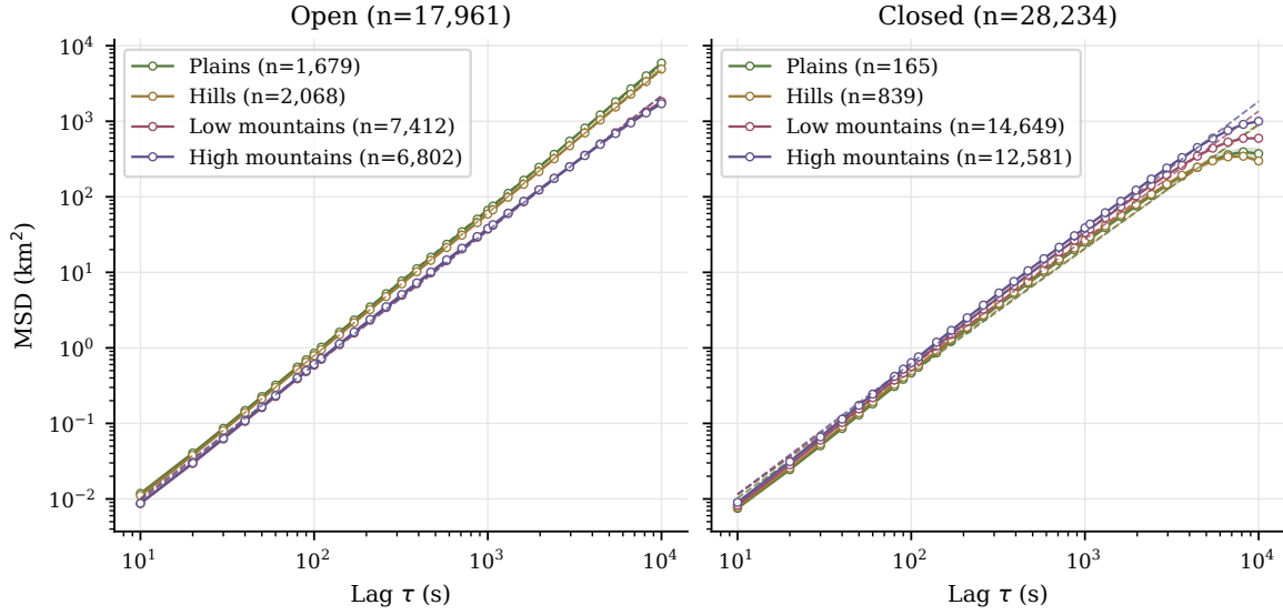
Figure 3.7. Paraglider transport by declared circuit and initial altitude, with fixed flights and segments throughout 10–10000 s. Markers give MSD estimates, shaded bands their pointwise 90% intervals, and dashed lines the global log–log fits. The identical axes permit comparison of displacement amplitude and growth rate.
