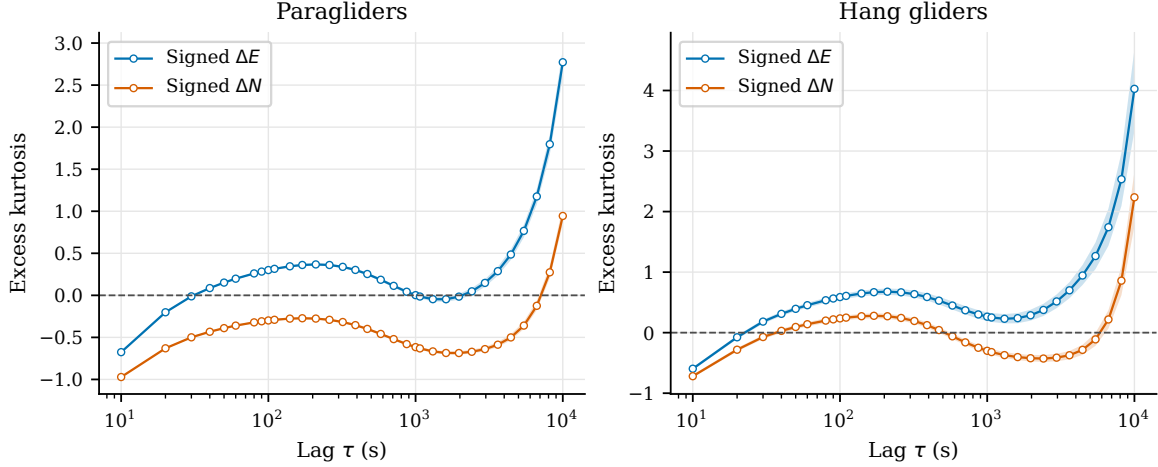
Figure 3.18. Signed-component Fisher excess kurtosis at the same lags, with the same flights, segments and weights as the quantiles and moments. The dashed line is the Gaussian marginal reference. Bands use the coupled cluster bootstrap.
