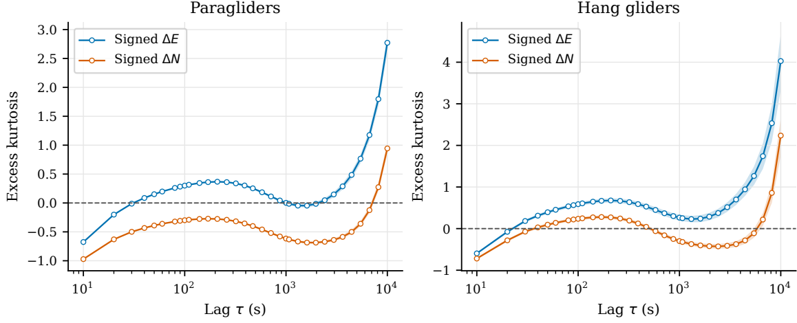
Figure 3.11. Signed-component Fisher excess kurtosis at the same lags, with the same flights, segments and weights as the quantiles and moments. The dashed line is the Gaussian marginal reference. Bands use the coupled cluster bootstrap.
