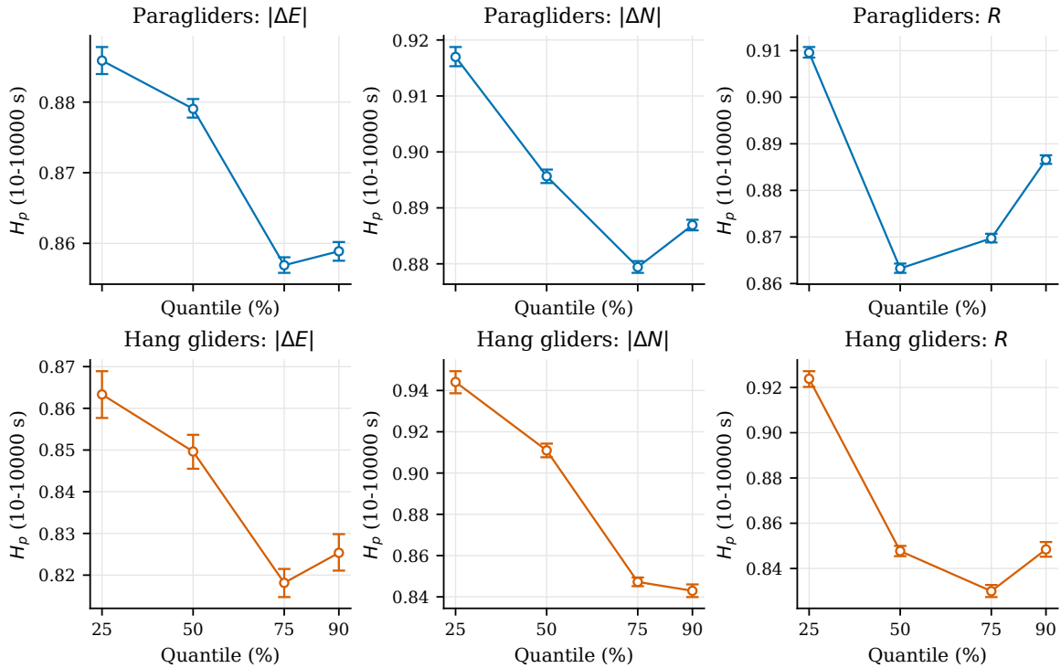
Figure 3.8. Global quantile exponents from 10–10000 s fits. Error bars are the 5th–95th percentiles of the refitted bootstrap slopes. A common scale exponent would give a horizontal sequence within each panel.
