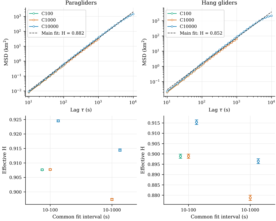
Figure 3.4. Effect of duration selection. Top: MSD in the three nested cohorts; dashed lines fit the main cohort over 10–10000 s. Bottom: effective H with 90% intervals, fitted over 10–100 s for all three cohorts and 10–1000 s for the two longer cohorts. Fits within each comparison use identical lag values.
