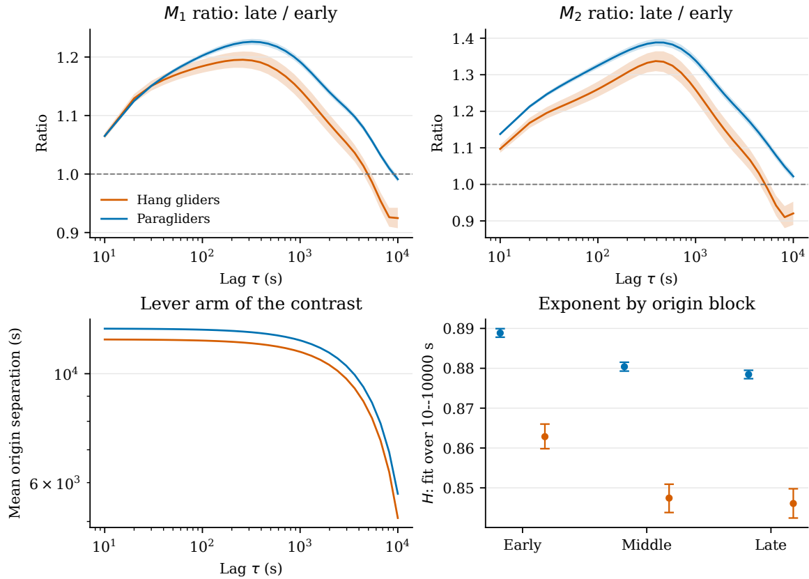
Figure 3.12. Origin dependence of the increment law in the main cohort. Top: the ratio of the late-block to the early-block radial moments, with 95% paired bootstrap bands and the stationary-increment value as a dashed line. Bottom left: the mean separation between the two blocks of origins, which shrinks as the lag consumes the segment. Bottom right: H fitted in each block over 10–10000 s. Bands and bars are pointwise.
