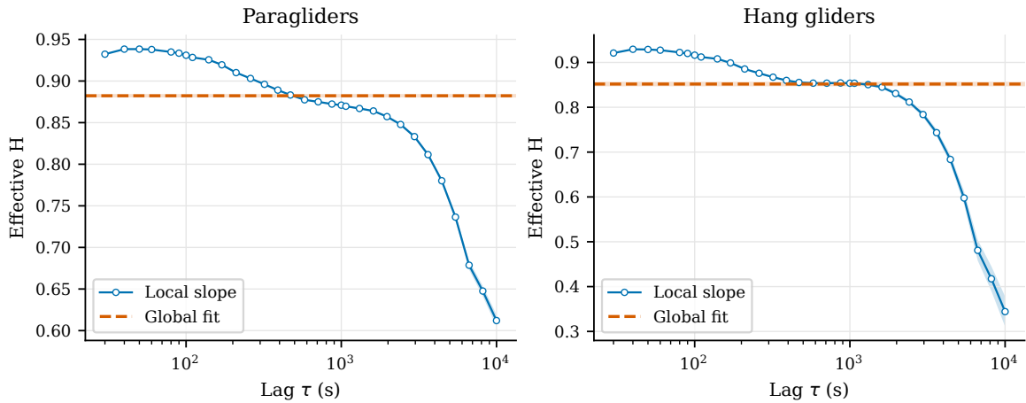
Figure 3.9. Local and global effective MSD exponents on the fixed main cohort. Bands are pointwise 90% bootstrap intervals. The global fit compresses the full curve into one number; the local slopes expose its scale dependence.
