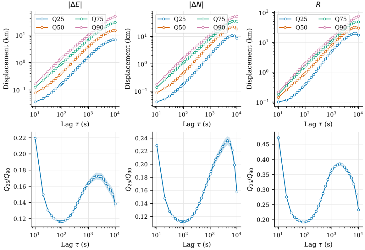
Figure 3.7. The same amplitude quantiles and ratio for hang gliders, with an independent main cohort and the same sampling convention.
