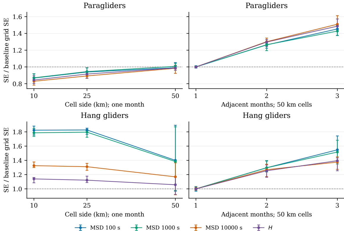
Figure 3.3. Standard errors relative to the unshifted 50 km, one-month grid baseline. Left: cell size and boundary shifts. Right: adjacent-month unions with seasonal boundary shifts. Markers are medians and bars span minima and maxima across partitions and two seeds; they are not confidence intervals. Altitude classes remain separate, and all years are pooled.
