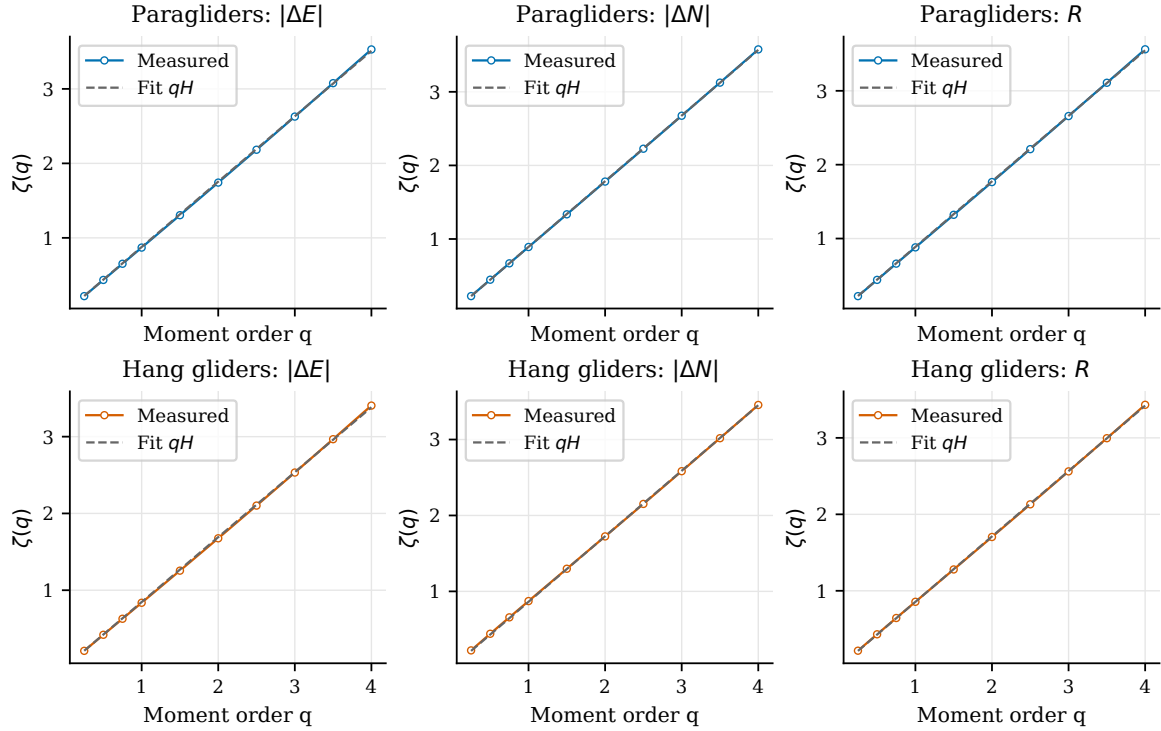
Figure 3.10. Moment spectra for the three displacement amplitudes. Each point is the slope of a 10–10000 s log–log moment fit; shading gives its pointwise 90% interval. Dashed lines are constrained linear fits \zeta = qH .
