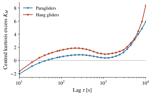
Centred, full-covariance Mardia excess; pooled windows. Positive excess does not identify a power-law tail. Mardia (1970).
