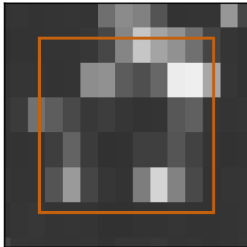
SEVIRI HRV, 1 x 2 km every 5 min, image of 12:30
