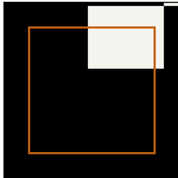
Cloud mask, white = cloud every 5 min, image of 12:30
