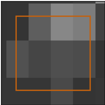
SEVIRI VIS0.6, 3 x 5 km every 5 min, image of 12:30
