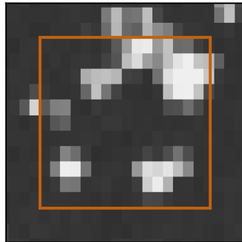
MTG VIS0.6, 0.6 x 0.9 km every 10 min, image of 12:30
