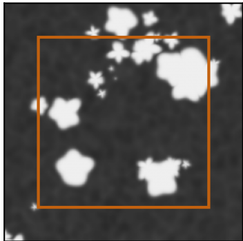
Synthetic cumuli (what is really there)
