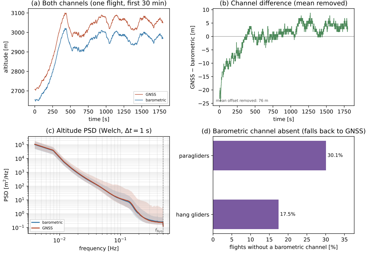
Figure 2.1: Barometric vs GNSS altitude noise. Panels (a)/(b): one representative flight over a 30 min window. (a) the two raw channels on a single shared axis, so their offset – the gap between the pressure and ellipsoidal references, tens of metres – is read directly, while both track the same vertical motion. (b) their difference GNSS–barometric (mean removed, not detrended): the offset drifts by tens of metres over the flight, a real feature – plausibly the barometric channel’s slow departure from the ICAO standard atmosphere as altitude changes – not noise, so only its constant part (annotated) is subtracted. Panels (c)/(d): over the ensemble. (c) the per-frequency median Welch spectrum of each channel (Appendix B), pooled over the two disciplines (whose spectra coincide), with a shaded 10 to 90 percentile band across flights. The median lines nearly coincide: for the typical flight the two channels are comparable at high frequency, both near the floor set by the shared metre-resolution logging. The relevant difference is in the bands : the barometric band stays tight (uniformly clean), whereas the GNSS band fans out by one to two orders of magnitude towards Nyquist, driven by a minority of flights with heavy multipath noise. The median is used rather than the mean because these per-flight spectra are heavy-tailed and a mean is dominated by that noisy minority (Sec. 2.6.1). The dotted line is the Nyquist frequency f_{Nyq} = 1/(2\Delta t) . (d) Fraction of flights whose barometric channel is absent, per discipline. (implementation details: Sec. 2.6.1)
