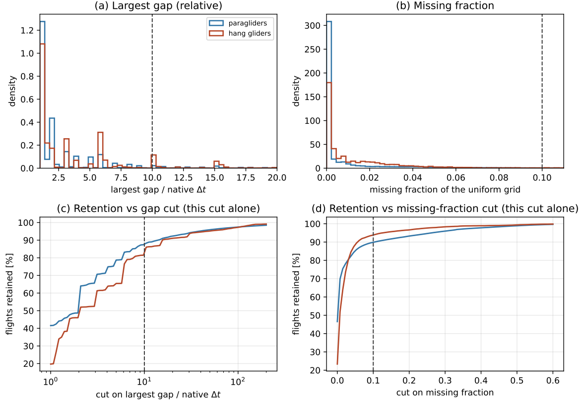
Figure 2.6: Sampling-regularity diagnostics, computed on the full dataset per discipline, on the same track scan as Figure 2.3 (so every parsed flight is included, not only the ones that survive the duration/path-length cuts). (a)/(b) Distribution of the largest single gap (relative to that flight’s own native \Delta t ) and of the missing fraction of a uniform grid at that interval, both on linear bins and a linear axis, over the bulk of the distribution (the heavy tail is not lost: (c)/(d) sweep the full range). Unlike native \Delta t (Figure 2.7) the largest-gap ratio is not purely discrete (a missed fix or two at the native rate is the most common cause of a large gap, but the gap’s exact duration is not grid-aligned to it), yet integer ratios (a gap of exactly k native intervals) are still visibly the dominant, common values, especially for hang gliders; a logarithmic axis, appropriate for a quantity spanning orders of magnitude, would have stretched precisely this small-integer structure into invisibility; the structure matters here because the adopted cut (dashed) sits on it. (c)/(d) The fraction of flights each cut would retain on its own (marginal, not cascaded), with the adopted thresholds marked; here the cut ranges over orders of magnitude to show the full saturating shape, so (c) keeps a logarithmic axis. (implementation details: Sec. 2.6.6)
