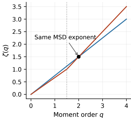
(a) Same MSD, different spectra
