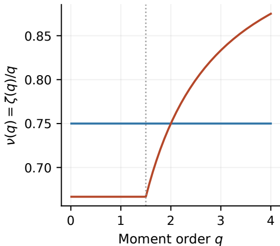
(b) Exponent per moment order
