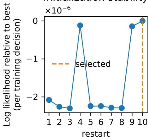
search: original covariance
