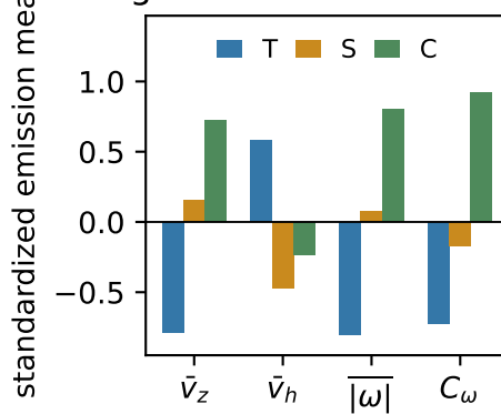
Original 4D emission means
