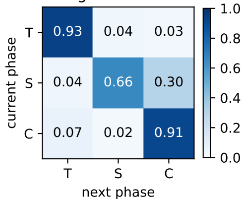
Initialization stability
