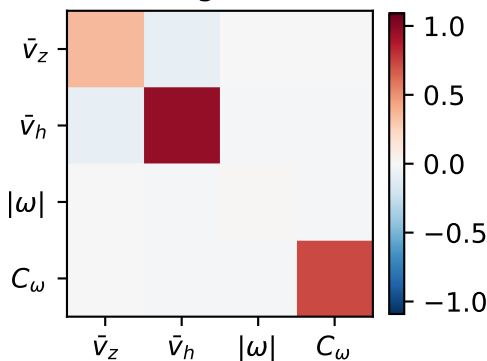
transition: original covariance
