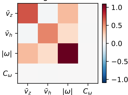
climb: original covariance
