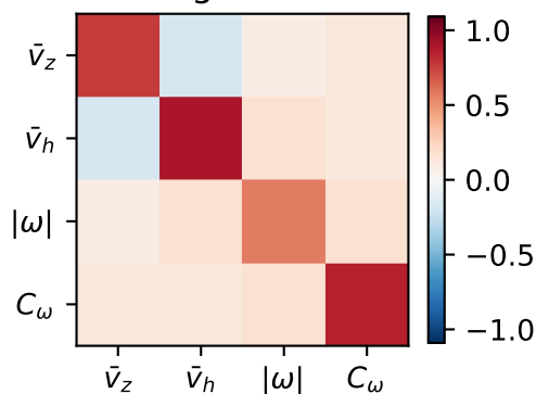
search: original covariance
