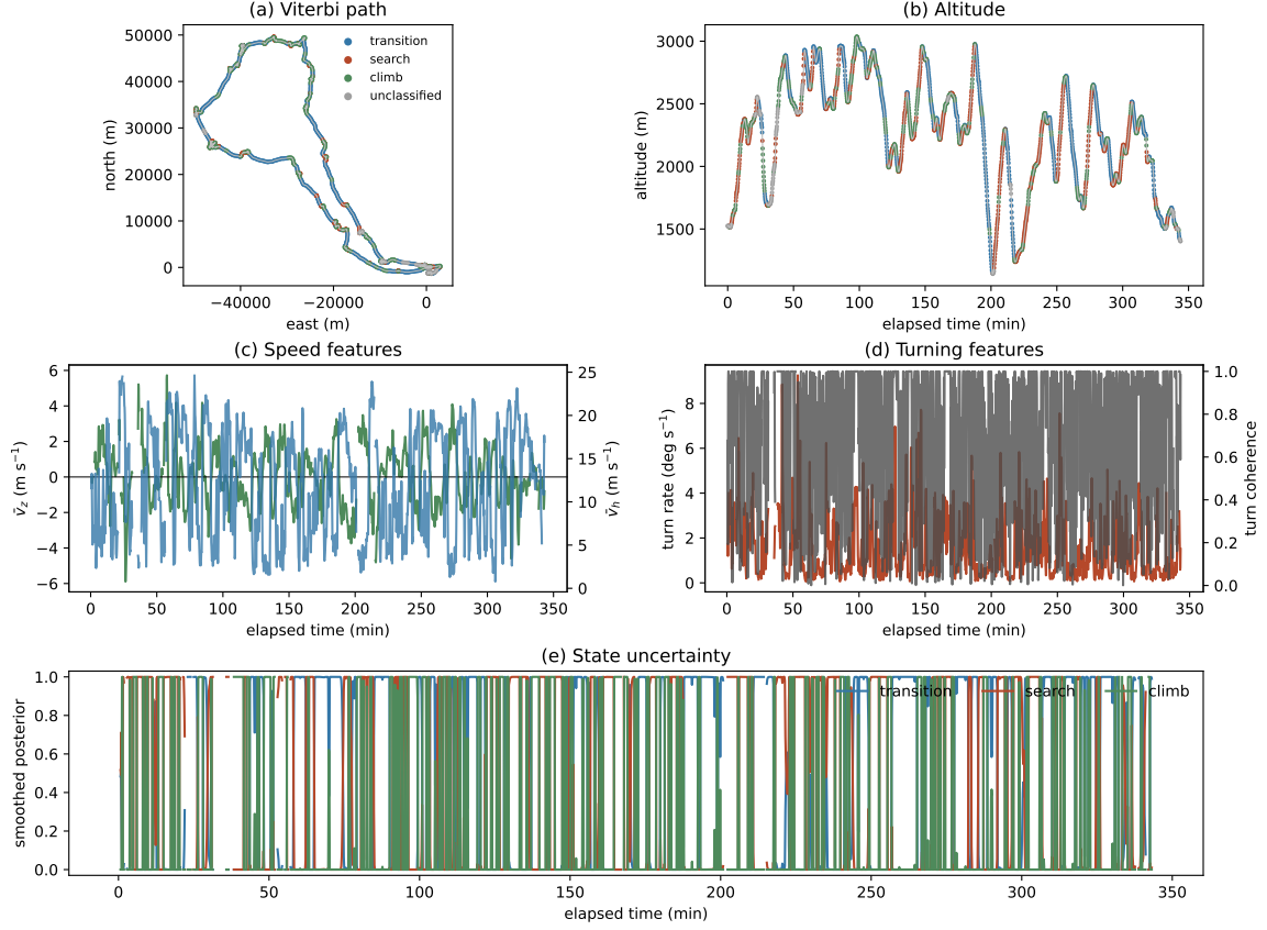
Figure 4.4. The corresponding held-out hang-glider trajectory diagnostic. Its HMM, standardizer and Viterbi path are independent of the paraglider model; colours retain the common provisional semantic convention to make the panels comparable.
