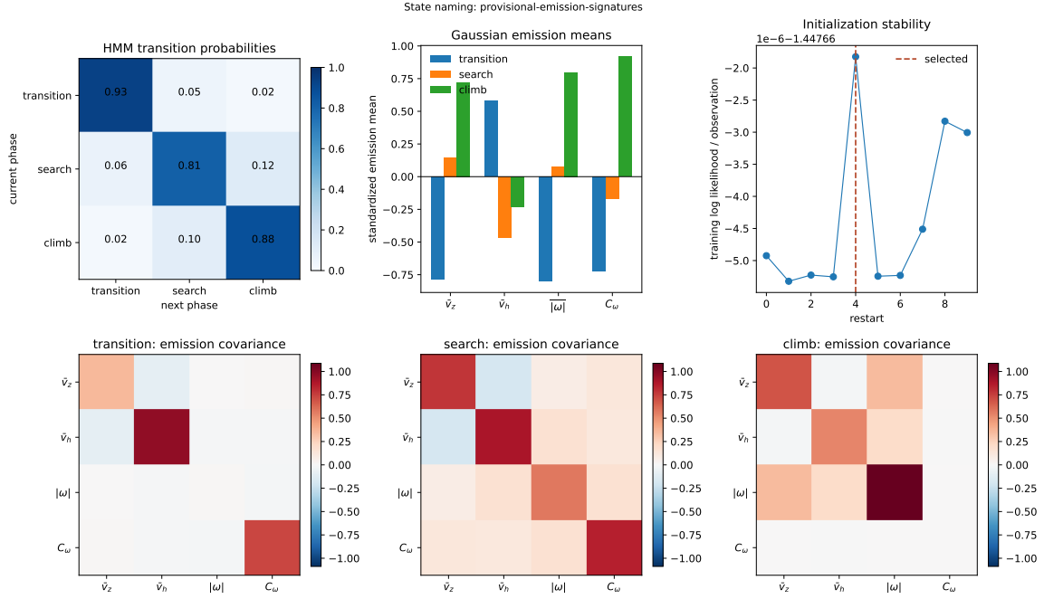
Figure 4.2. Fitted hang-glider HMM diagnostics, with the same quantities, ordering and provisional state-naming convention as Fig. 4.1. The separate emission and transition parameters are essential: no fitted parameter or scaler is shared between disciplines.
