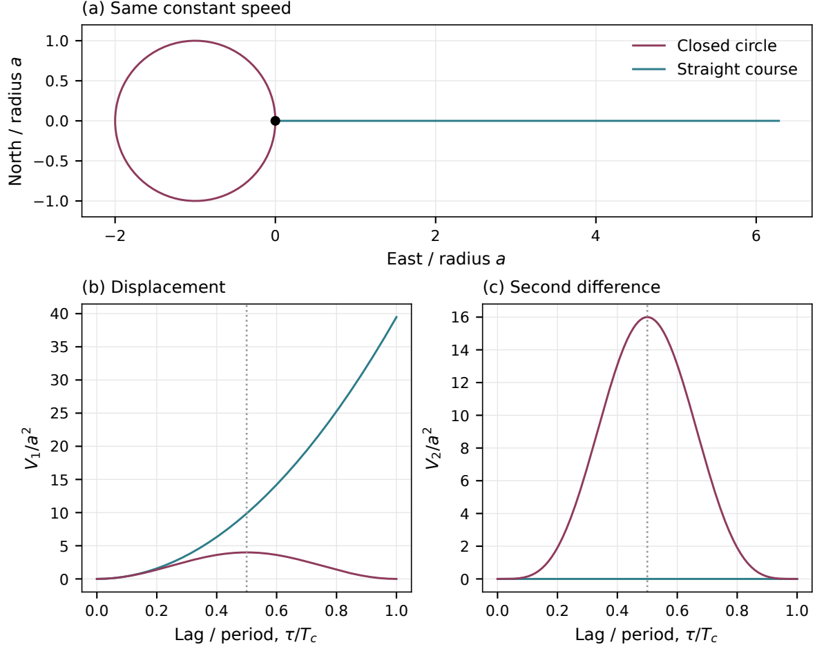
Figure 3.3. Analytical straight and circular paths at the same speed. The circle is continued periodically to evaluate second differences. Both V_1 and V_2 vanish after a complete period: constant-velocity removal preserves the effect of route closure.
