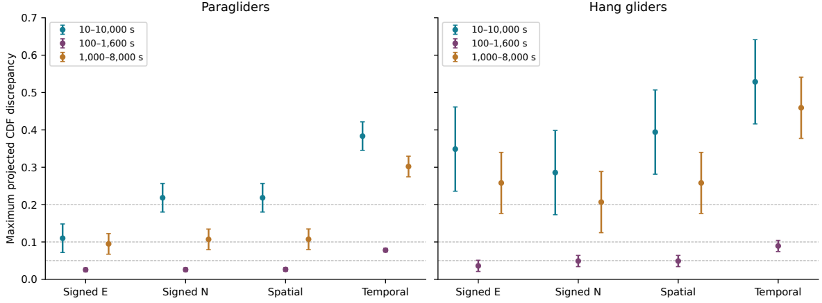
Figure 3.14. Held-out projected-CDF discrepancies and simultaneous 95% bootstrap bounds. Dashed lines mark the declared tolerances. One common training exponent rescales all four coordinates. Each grid retains its own fixed population.
