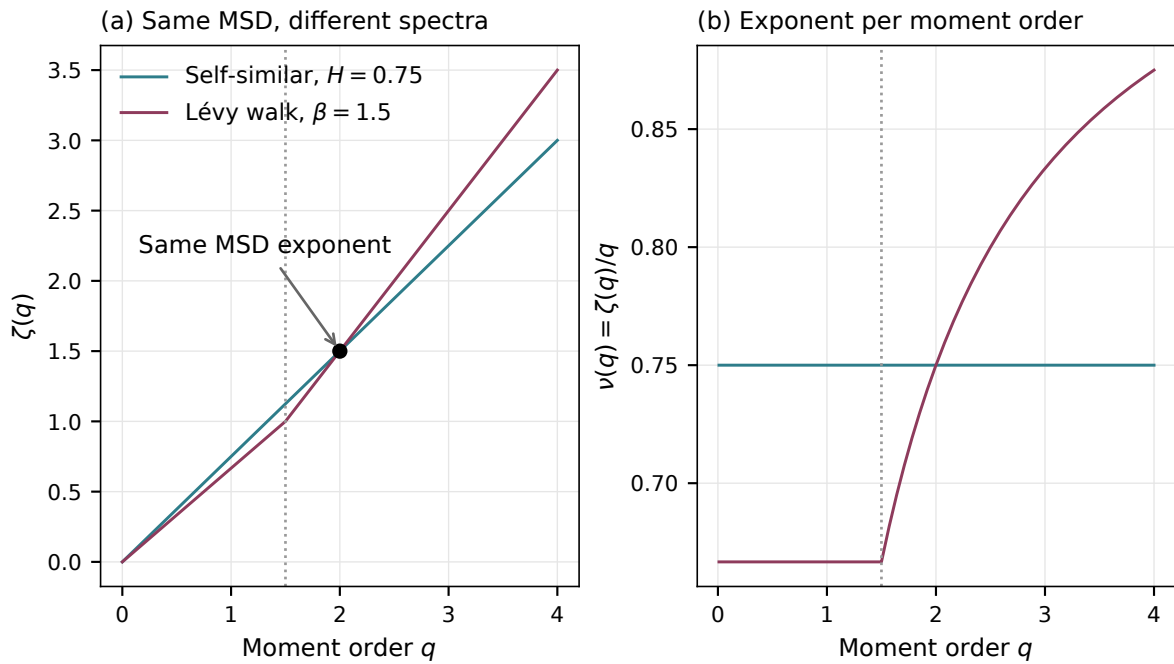
Figure 3.36. Theoretical comparison. A self-similar process with H = 0.75 and a standard Lévy walk with \beta = 1.5 have the same MSD exponent, \zeta(2) = 1.5 , but different moment spectra. The dashed vertical line marks q = \beta . These are asymptotic predictions, not simulated or empirical estimates.
