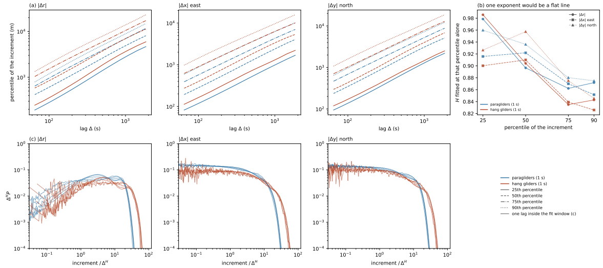
Figure 3.3. The exponent read from the distribution of the increments, not from a moment of it. All seven panels use each discipline’s fastest native cadence, 1 s, where the histograms hold the most increments. (a) The 25th, 50th, 75th and 90th percentiles against lag, log–log, over the fit window 60 s to 2,000 s, one column for the modulus |\Delta \mathbf{r}| and one for each horizontal component. Four parallel lines would mean one exponent describes every part of that column’s distribution. (b) The slope of each of those four lines, fitted separately, with the modulus and the two components overlaid in one panel rather than split into columns — it is already the comparison across variables that (a) and (c) split apart. A flat line would mean the same thing as in (a). All three fall from the 25th percentile to the 90th, so the disagreement is not a property of one direction. (c) The histograms behind each column of (a), rescaled by \Delta^H , one curve per lag inside the fit window and every third lag drawn. H is that column’s own value: 0.884 (modulus), 0.893 (east), 0.908 (north) for paragliders, and correspondingly 0.873, 0.870, 0.901 for hang gliders — not a value shared across columns, since H differs by component. If the scaling form held exactly the curves of one column would lie on top of one another; they do through the bulk and separate at the flanks, in every column.
