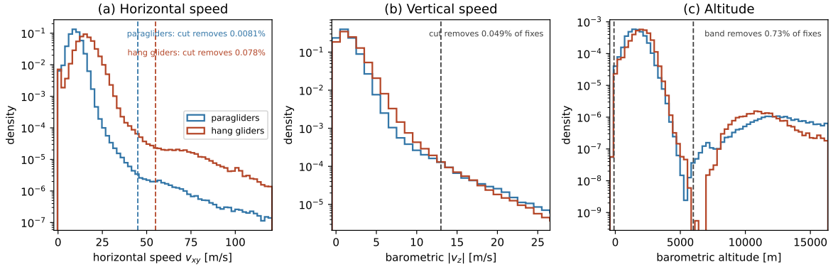
Figure 2.2. Fix-level cleaning: auditing the absolute bounds. Per-fix distributions of the quantities the out-of-range bounds test – (a) horizontal speed v_{xy} , (b) barometric |v_z| , (c) barometric altitude – pooled over a large paraglider subsample and the complete hang-glider population, with the adopted bounds dashed (Table 2.3); the y -axis is logarithmic so the sparse tail the bounds act on is visible. Panel (a) shows why the speed bound is per-discipline: hang gliders carry a non-decaying plateau of implausible sustained ground speeds ( 55 \text{ m s}^{-1} to 90 \text{ m s}^{-1} ), and the bound sits where the real decay stops. Binning choices, sample sizes and the validation of the robust detectors: Sec. 2.6.2. (implementation details: Sec. 2.6.2)
