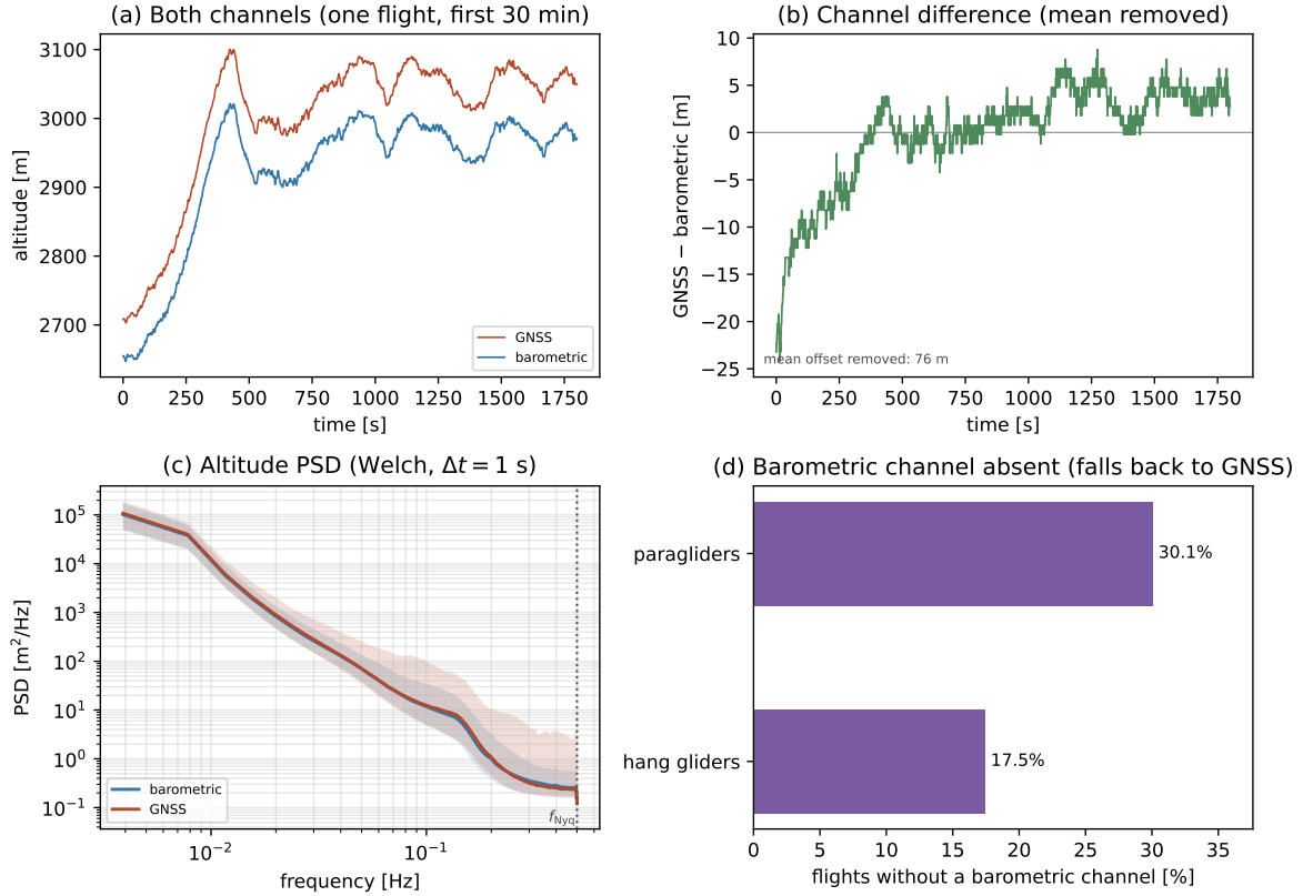
Figure 2.1. Barometric vs GNSS altitude noise. (a) One representative flight over a 30 min window: the two raw channels on a shared axis; the gap between them is the offset between the pressure and ellipsoidal references. (b) Their difference, mean removed: the offset also drifts by tens of metres over the flight, so only its constant part (annotated) is subtracted. (c) Per-frequency median Welch spectrum of each channel (Appendix B), pooled over the two disciplines, with the 10 to 90 percentile band across flights; the medians nearly coincide, while the GNSS band fans out towards the Nyquist frequency f_{\text{Nyq}} = 1/(2\Delta t) (dotted). The median is used because the per-flight spectra are heavy-tailed (Sec. 2.6.1). (d) Fraction of flights whose barometric channel is absent, per discipline. (implementation details: Sec. 2.6.1)
