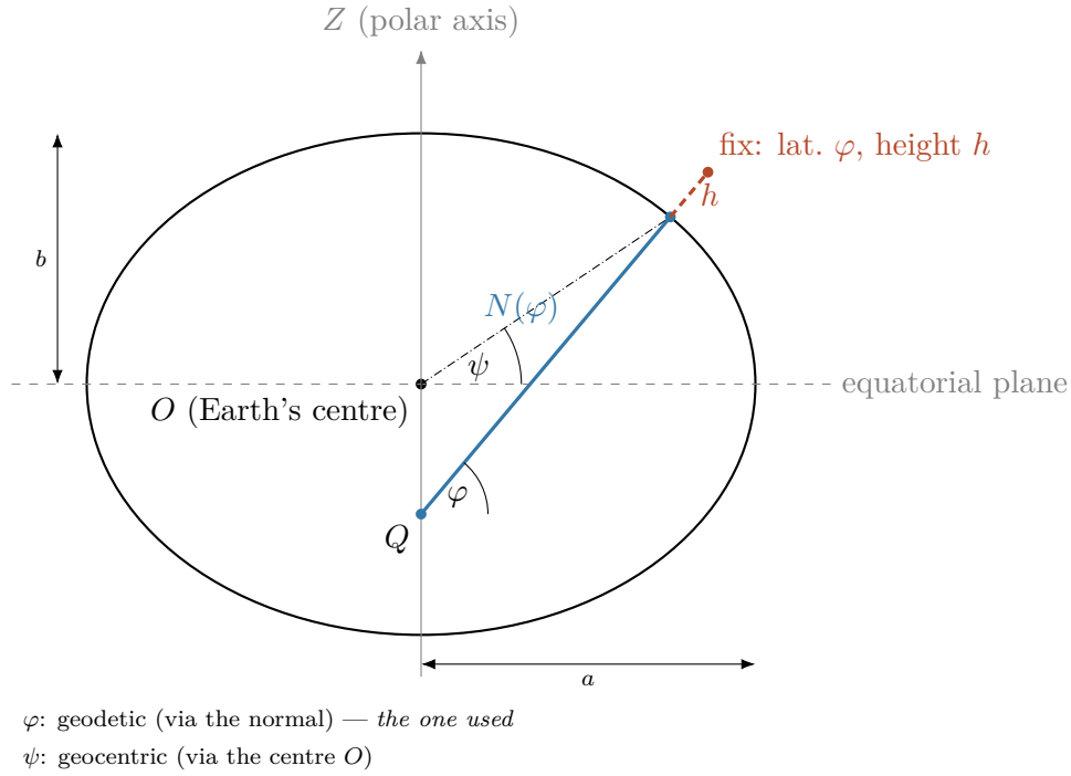
Figure 2.4. Geodetic latitude and height on the reference ellipsoid, in meridian cross-section (flattening exaggerated; the true WGS84 f \approx 1/298 would be indistinguishable from a circle): the semi-axes a and b ; the geodetic latitude \varphi , the angle between the ellipsoid normal and the equatorial plane; the height h along that normal; and N(\varphi) , the distance along the normal from the surface to the point Q on the polar axis. The normal does not pass through the centre O , so \varphi differs from the geocentric latitude \psi (dash-dotted). Longitude \lambda is out of the page here; it is shown in Figure 2.5.
