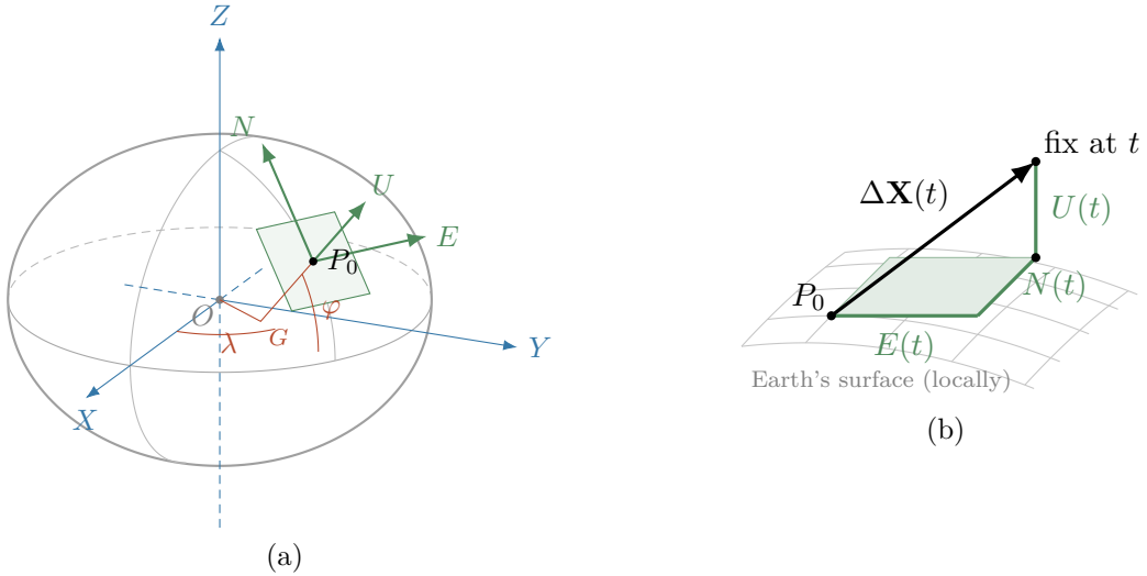
Figure 2.5. The ENU rotation. (a) The global ECEF frame ( X, Y, Z ) in blue, centred at the Earth’s centre O ; the two red angles that locate the take-off fix P_0 : longitude \lambda , measured in the equatorial plane from the prime meridian, and geodetic latitude \varphi , the tilt of the ellipsoid normal, measured at the point G where the normal meets the equatorial plane; and the local ENU frame in green, tangent at P_0 . Flattening exaggerated as in Figure 2.4: U follows the normal G-P_0 , not the radius from O . The green arrows are the rows of the rotation matrix, as unit vectors. (b) Close-up of the tangent plane: a later fix’s ECEF displacement \Delta \mathbf{X}(t) is the space diagonal of the box whose edges are its ENU components E(t) , N(t) , U(t) .
