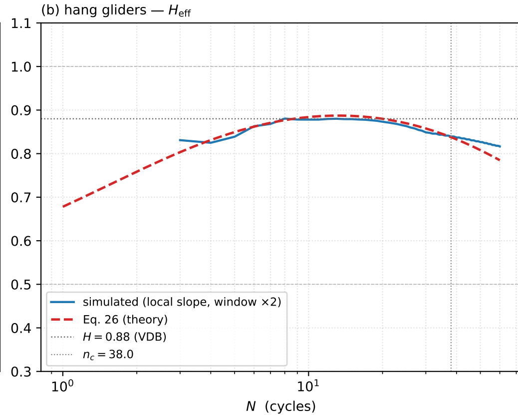
Cycle-counted effective Hurst exponent: simulation vs paper Eq. 26
