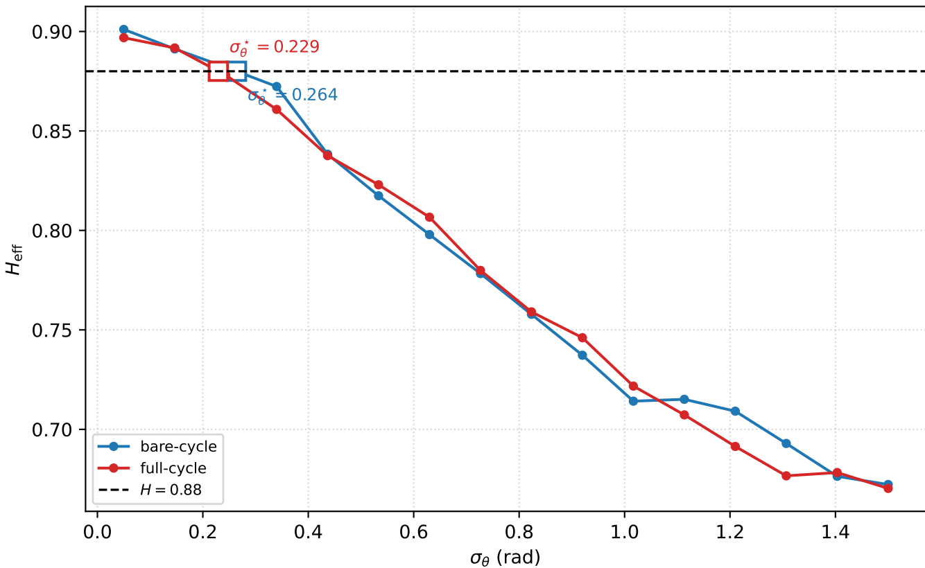
H_{\text{eff}}(\sigma_\theta) — hang gliders (fit window [10, 7000] s)
