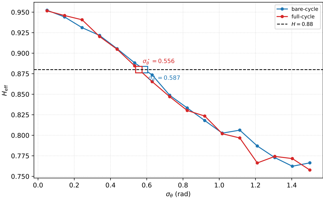
H_{\text{eff}}(\sigma_\theta) — sailplanes (fit window [10, 7000] s)
