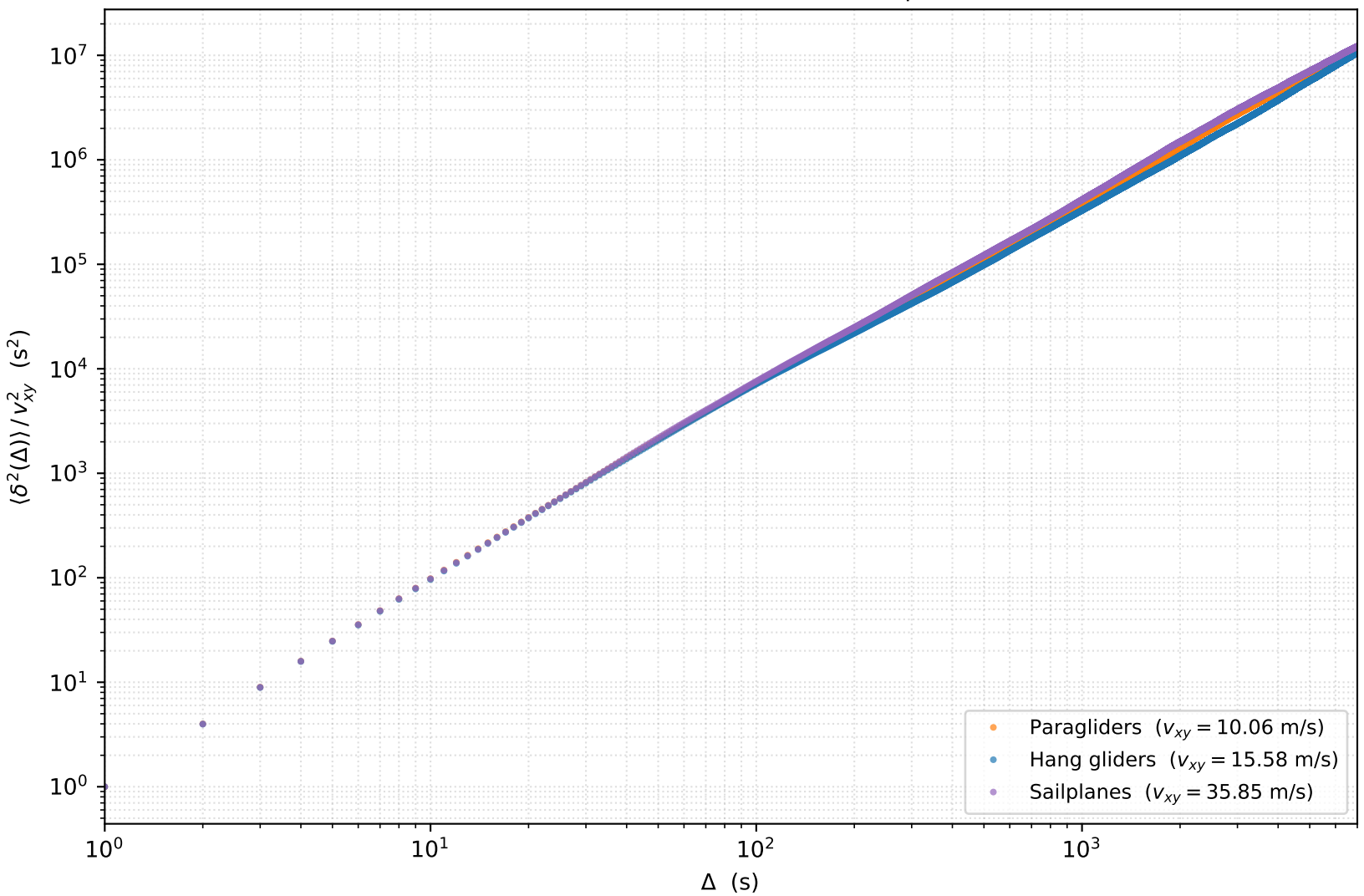
Rescaled MSD — universal collapse
