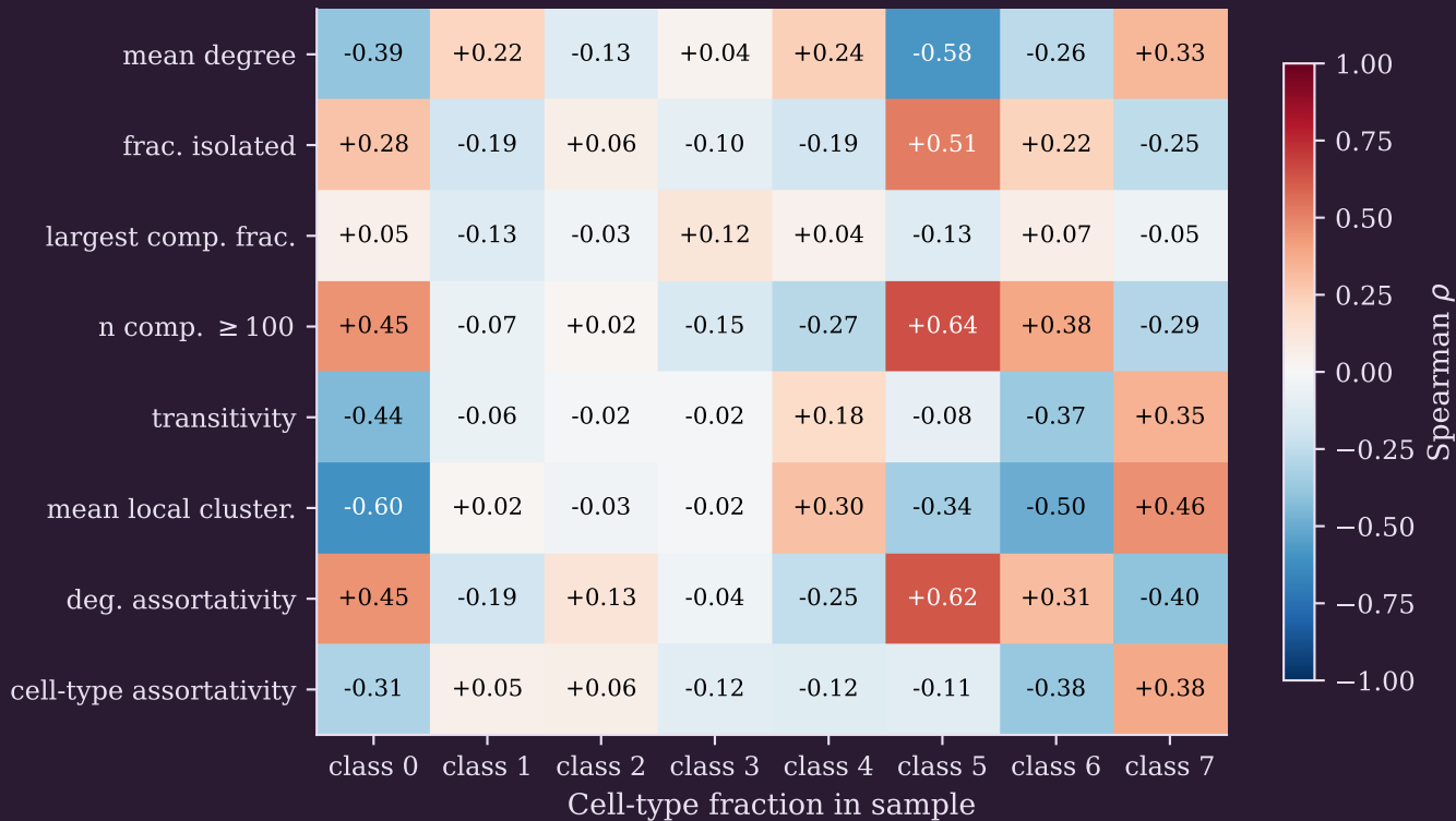
Spearman correlation: topology metrics \times cell-type composition (n = 110)
