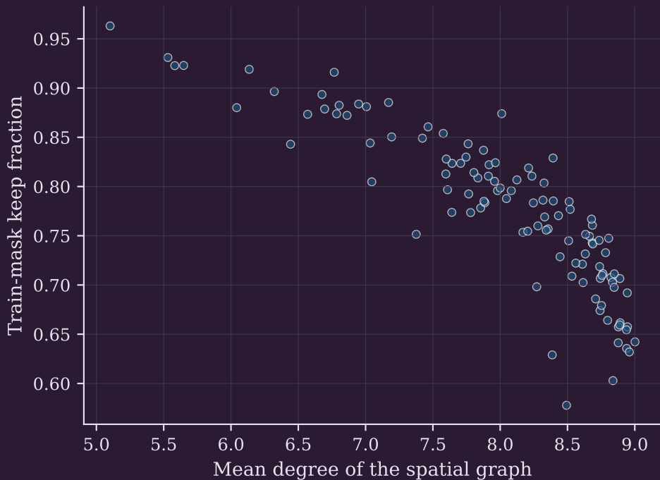
Train mask is a function of local density Spearman \rho = -0.91
