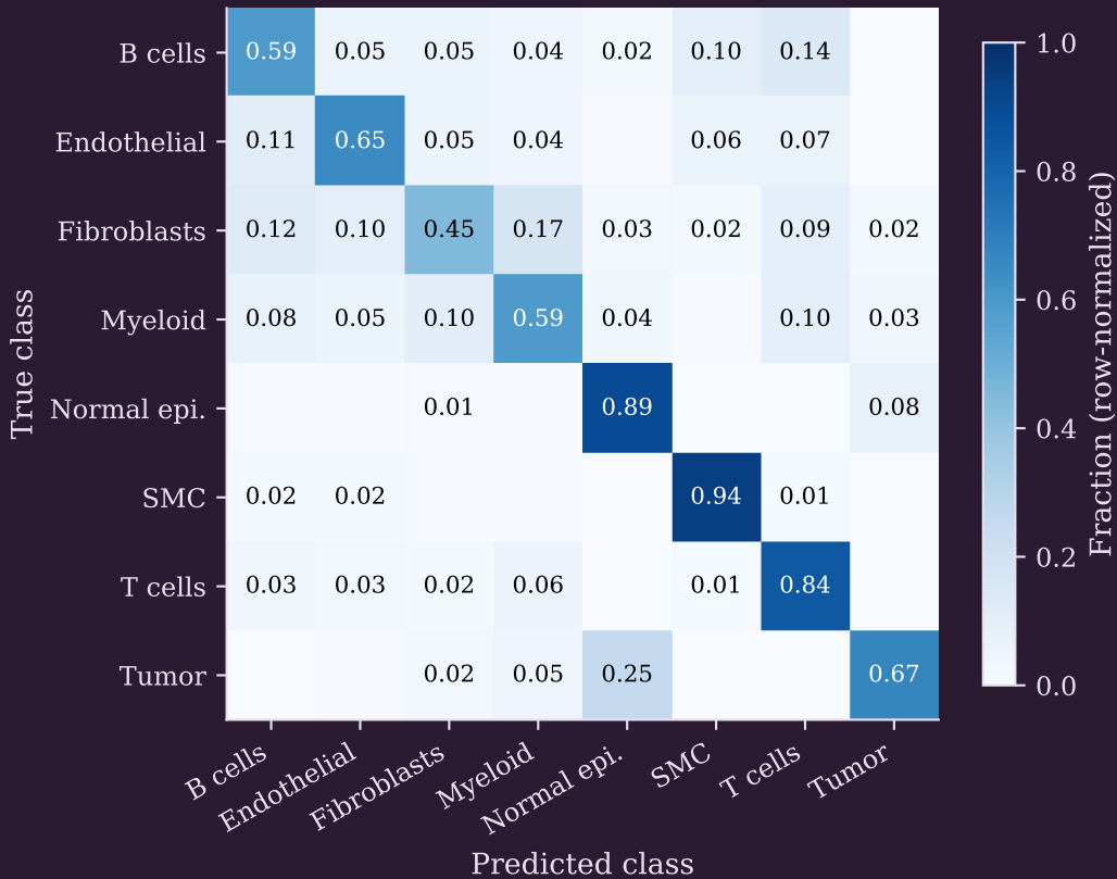
Rung 3 test set: row-normalized confusion matrix
